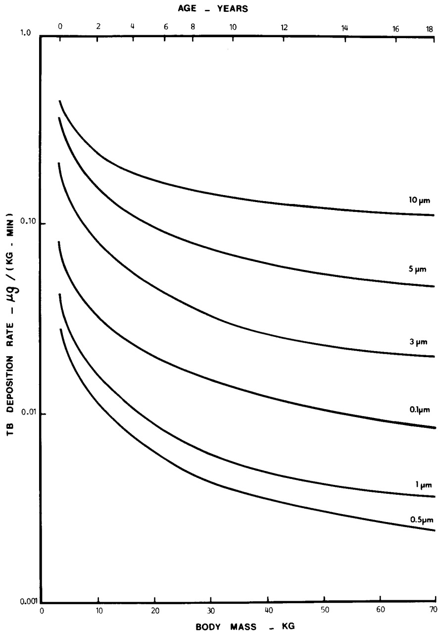
Fig. 8. Predicted initial dose to the tracheobronchial region as a function of body mass. Assumptions include equivalent upper airway deposition for all ages, inhalation of particles at 1 \text{ mg/m}^3 concentration in air, and resting minute ventilation V_m . The equation used to generate the curves was: D_{TB} = V_m (\text{m}^3/\text{min}) P_{TB} 1 (\text{mg}/\text{m}^3)/\text{body mass (kg)} , where P_{TB} is the appropriate tracheobronchial deposition efficiency.
