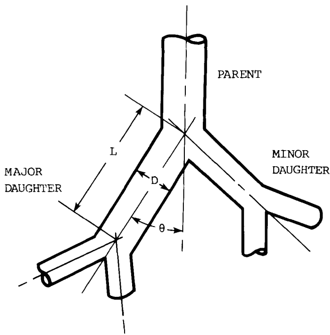
Fig. 1. Idealized airway branch showing parameters measured morphometrically on airway casts.
