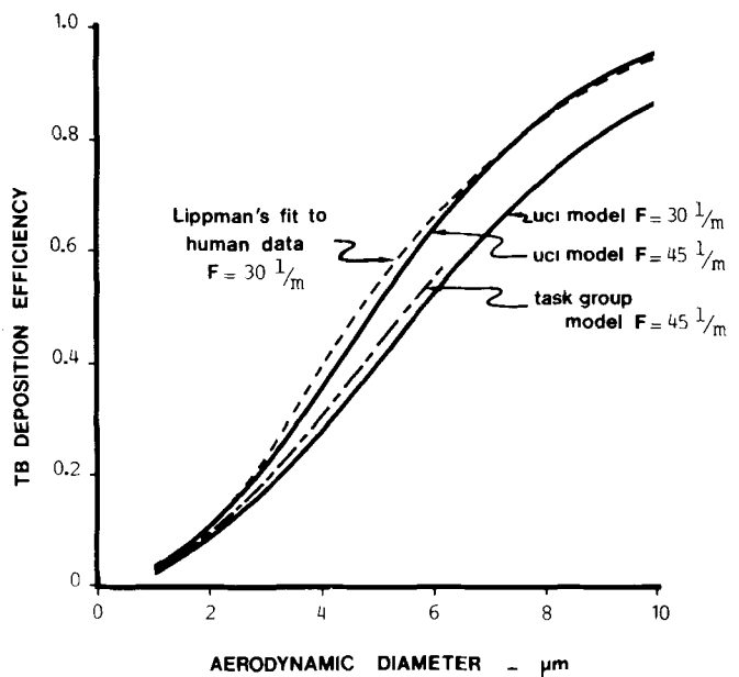
Fig. 7. Comparison of model predictions for tracheobronchial deposition efficiencies (as fraction of number entering trachea) for particles. Lippmann's curve is an empirical fit to data acquired from nonsmoking adults (Lippmann et al., 1971; Chan and Lippmann, 1980). The Task Group curve is theoretical (Task Group on Lung Dynamics, 1966). Two of our (UCI) computed curves are shown. The flows given are twice the minute ventilation. Values reported by Stahlhofen et al. (1981) are not included because of uncertainties in mouth deposition, but these values tend to fall below those shown.
