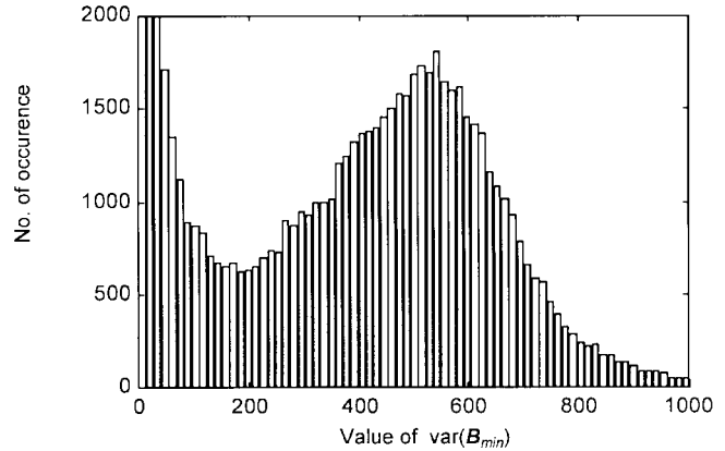
Fig. 3. Histogram of \text{var}(B_{\min}) .
