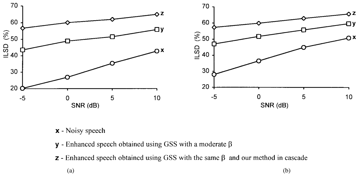
Fig. 5. Graphs of ILSD measurements versus SNR for (a) WGN and (b) computer fan noise.
