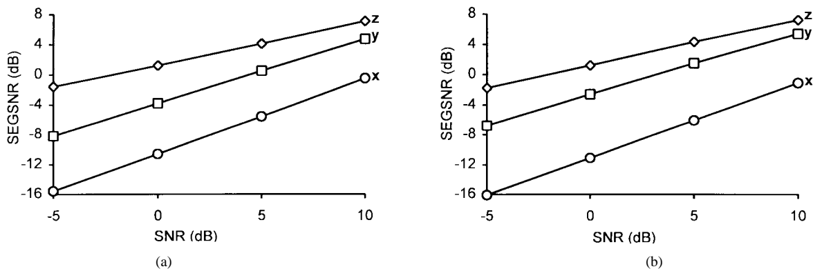
Fig. 6. Same as Fig. 5 except that SEGSNR instead of ILSD is used.
