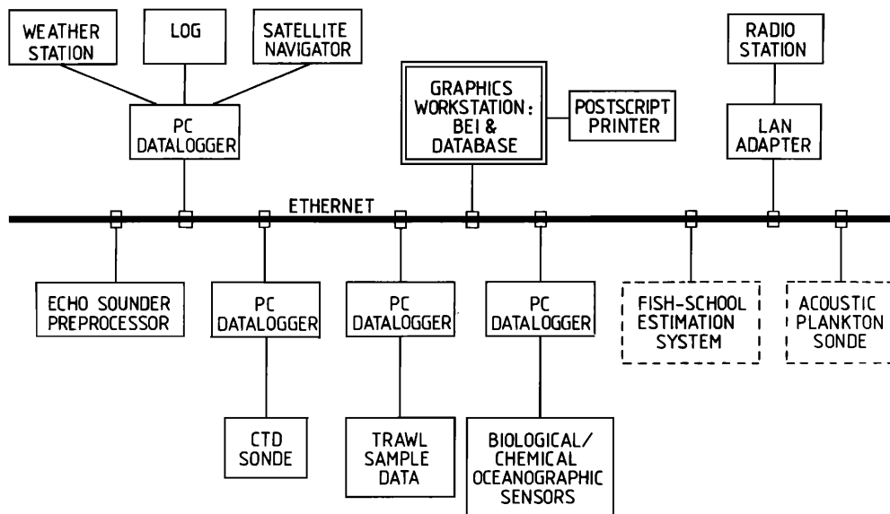
FIG. 1. Data network for research vessels.
