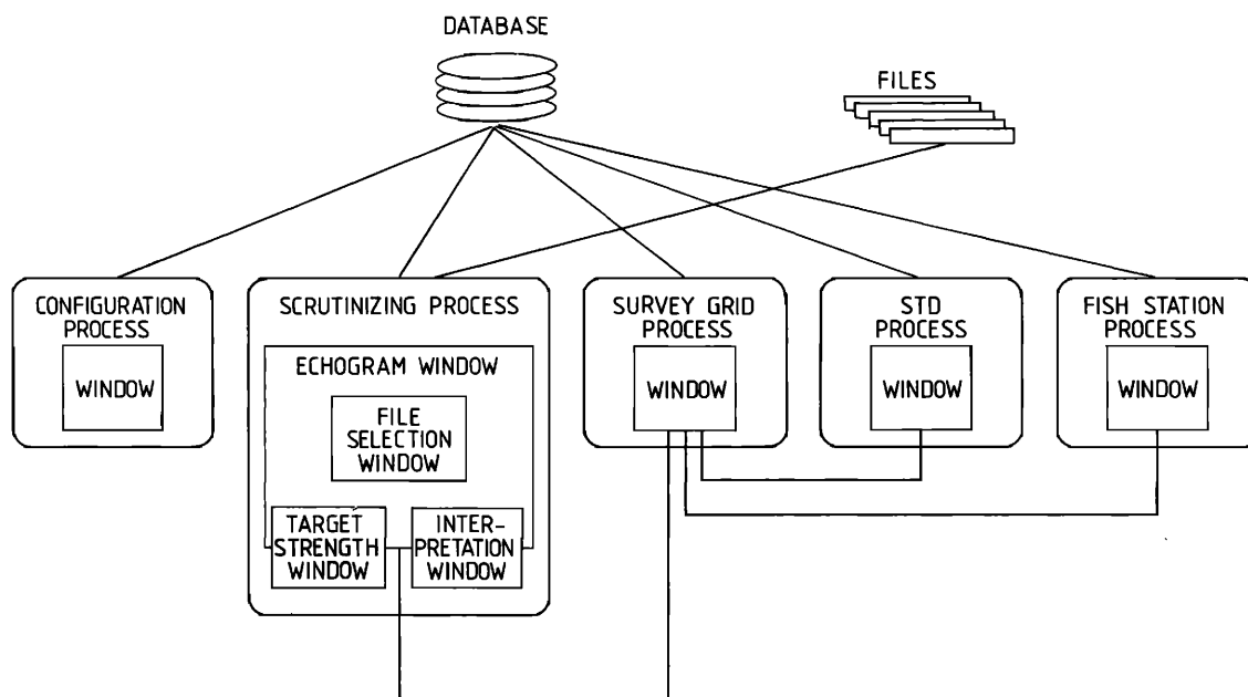
FIG. 4. Interconnections of graphical user interfaces and stored data.
