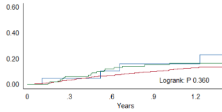
Kaplan-Meier failure estimates
