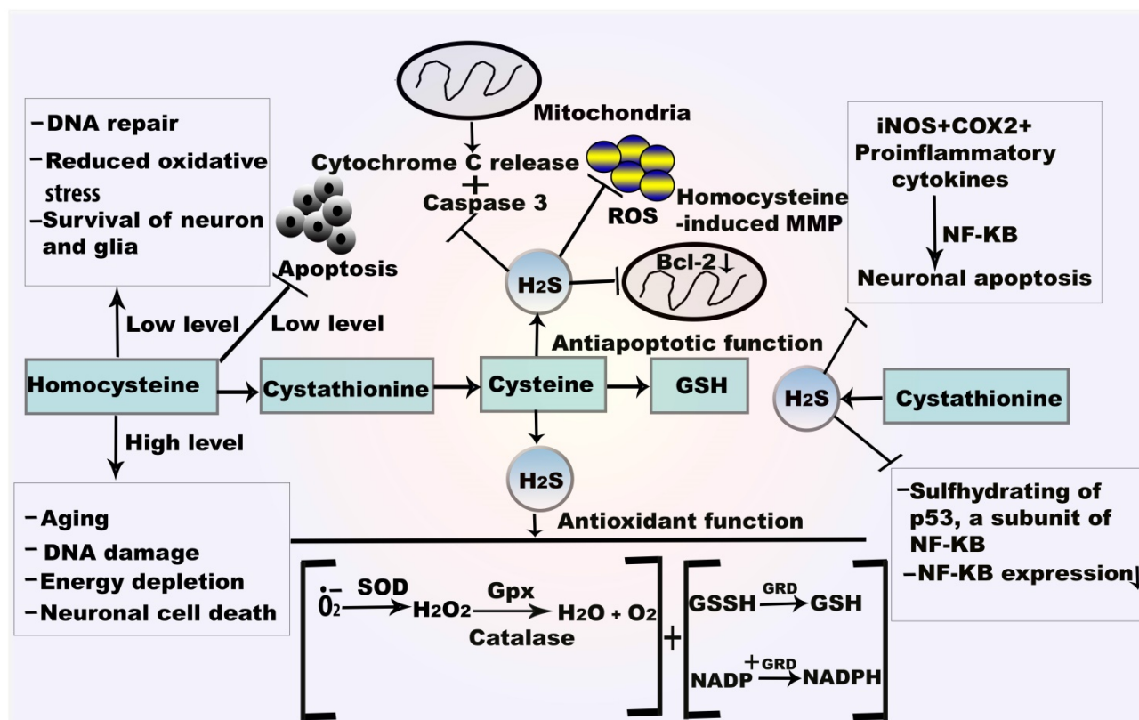
Figure 2. Mechanism of H 2 S in autoxidation and antiapoptosis. GSH reacts with oxygen free radical which directly form the thiol radical and later GSSH. SOD catalyses the dismutation of O 2 - and converted to H 2 O and O 2 . H 2 O 2 is also attenuated by the catalysis of CAT and Gpx. H 2 S also provides antiapoptotic function by NF- \kappa B and caspase 3. H 2 S from CSE plays role in sulfhydrating the p65 subunit of NF- \kappa B at cysteine 38. Abbreviations: GSSH, oxidized glutathione; GRD, glutathione reductase; NF- \kappa B, nuclear factor kappa B.
