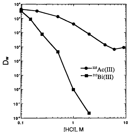
Fig. 2. Acid dependency of weight distribution coefficient of silica Ac-Resin for ^{225}\text{Ac(III)} and ^{213}\text{Bi(III)} at 25°C.
