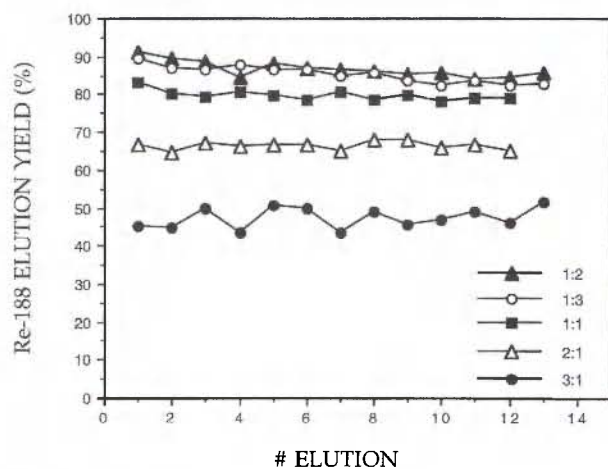
Fig. 4. Effect of various molar ratios of zirconium to tungsten on Re-188 elution yield vs. elution number.
