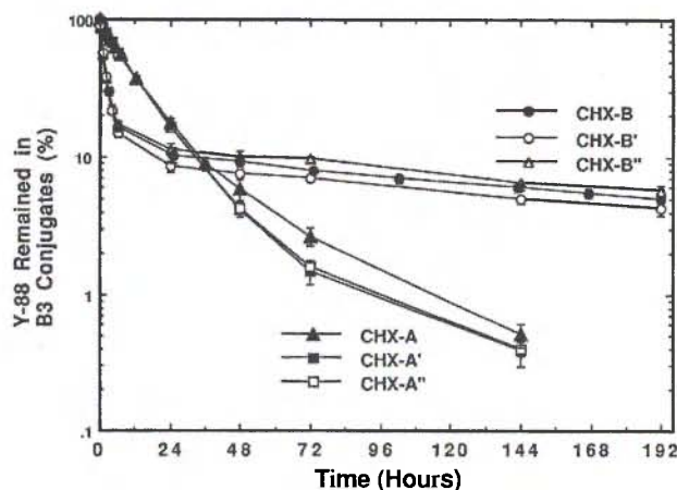
Fig. 4. Transchelation of 88 Y from 88 Y-CHX-DTPA monoclonal antibody B3 conjugates.
