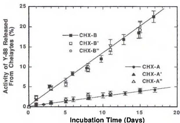
Fig. 3. Serum stability of 88 Y-CHX-DTPA complexes.
