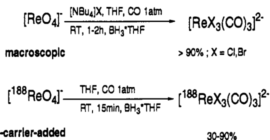
Scheme 1. Synthesis of [MX 3 (CO) 3 ] 2- under ambient conditions.
