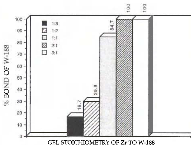
Fig. 5. Percentage of incorporated W-188 into insoluble zirconium tungstate gel at various gel stoichiometries.
