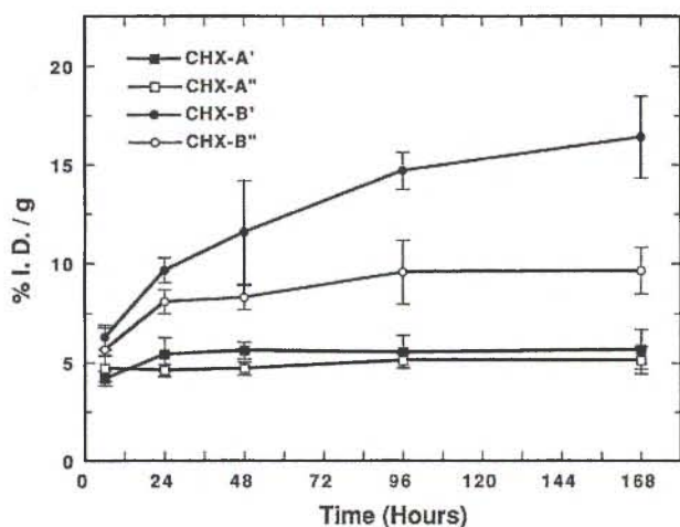
Fig. 5. ^{88}\text{Y} bone uptake from ^{88}\text{Y} -CHX-DTPA monoclonal antibody B3 conjugates in mice.
