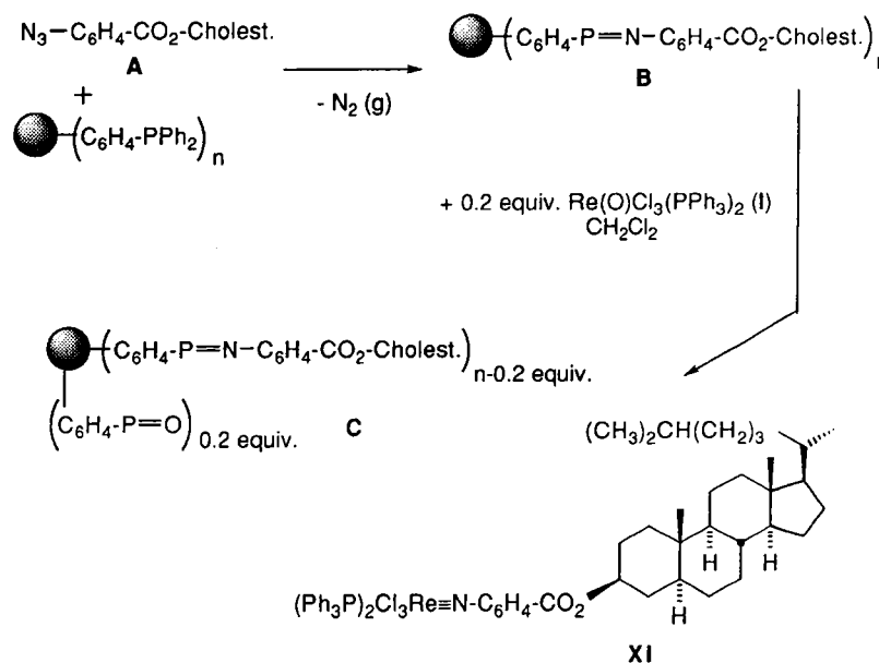
Scheme 2. Synthesis of a rhenium imido-cholesterol complex from a solid support.
