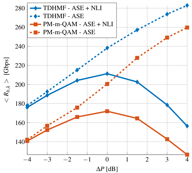
Fig. 5. \langle R_{b,\lambda} \rangle vs \Delta P for the two considered modulation strategies. R_{b,\lambda} has been averaged over N_{MC} = 2500 Monte Carlo runs.
