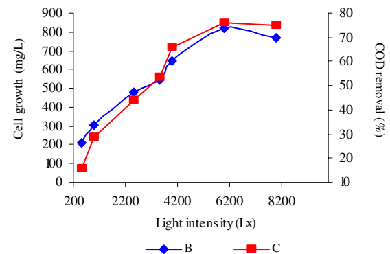
Fig. 5: Effect of light intensity variation on % COD removal and cell growth (mg/L). C = % COD removal, B = Cell growth
