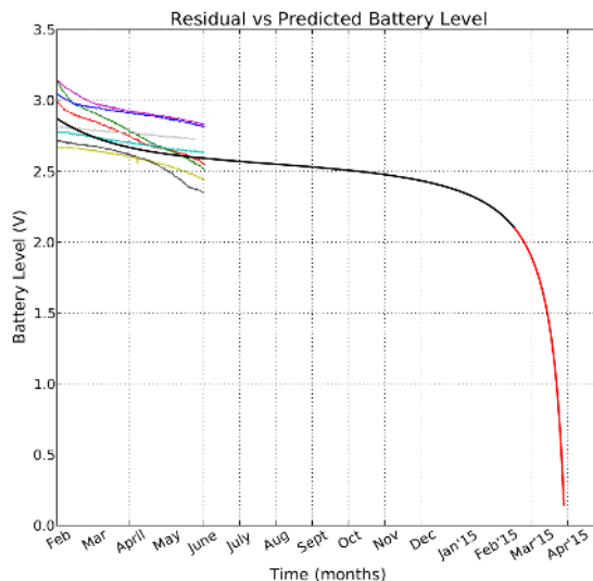
Fig. 11. Simulated battery discharge curve
