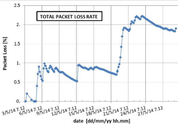
Fig. 8. Total packet loss ratio
