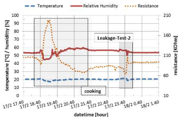
Fig. 5. Second leakage test with standard sampling technique
