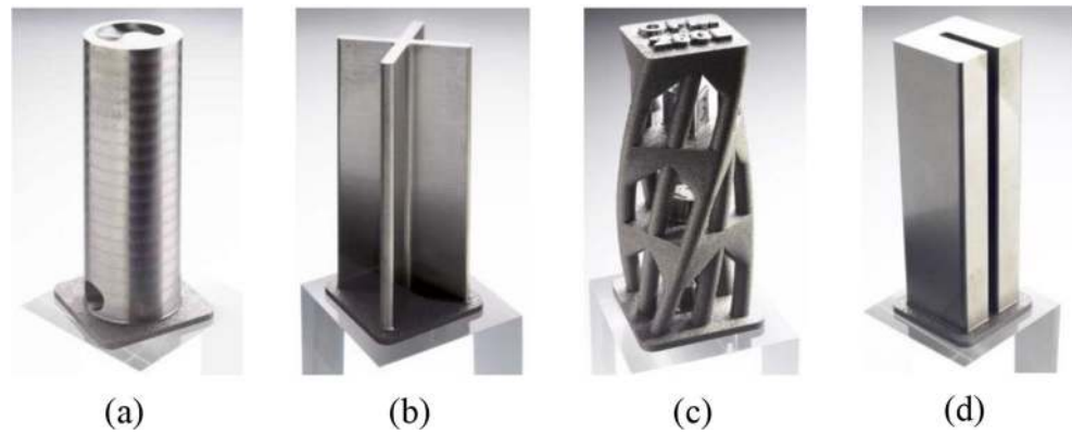
Fig. 20 Hybrid AM parts produced with Sodick's new OPM250L machine that combines LPBF with milling operations [161]
