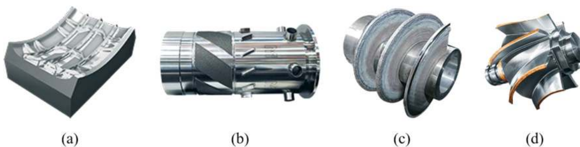
Fig. 23 Hybrid AM applications of the Mazak Integrex i-400AM system. a A mould insert. b, c General machinery. d Surface coating added to an impeller [164]
