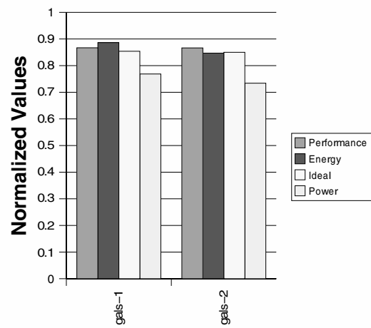
Figure 13. Impact of selective fetch and FP clock slowdown (gcc benchmark)
