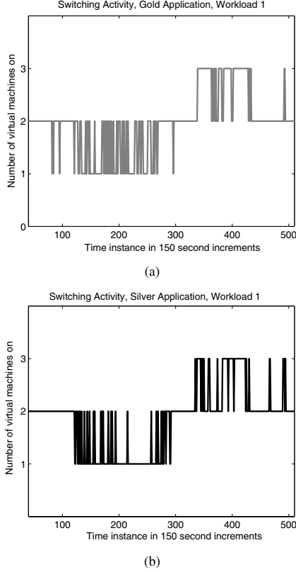
Fig. 10. The number of virtual machines assigned to the Gold and Silver applications processing Workload 1.
