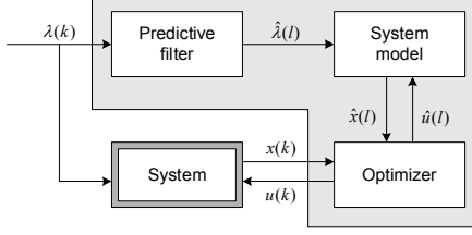
Fig. 5. The schematic of a limited lookahead controller.
