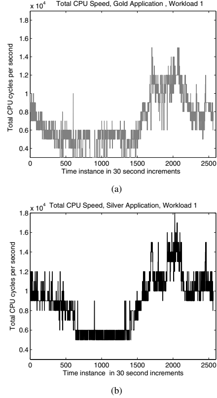
Fig. 11. CPU cycles assigned to the Gold and Silver applications under Workload 1.
