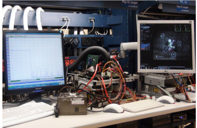
Figure 5: Experimental setup of a quad core Intel® Core™ 2 Duo 2860QM system
