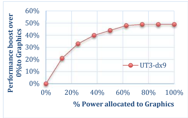
Figure 8: Power budgeting between CPU and Processor Graphics
