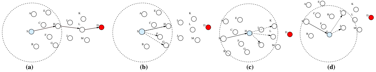
Fig. 10. Example for GPSR and MGPSR.
