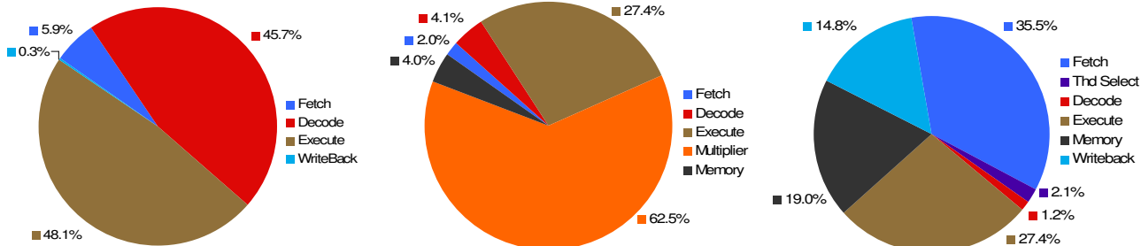
Figure 3: Power imbalance is common in many processor pipelines (even simple, in-order pipelines). On average, the ratio of power consumption between the most power-hungry stage and the least power hungry stage is over 150 for the Rigel pipeline (left) and over 30 for the OpenMSP430 (middle) and OpenSPARC T1 (right) pipelines.
