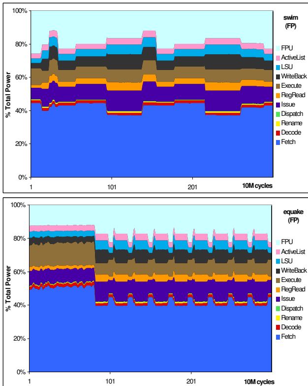
Figure 13: Dynamic changes in the power breakdown of a processor while running a FP benchmark do not deviate significantly from the average. Results are shown for the FP benchmarks that exhibit the most dynamic variation.
