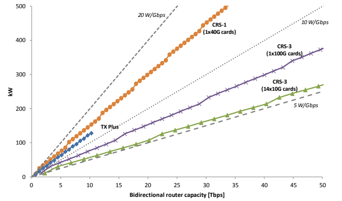
Fig. 3 Core router power consumption as a function of the total node capacity, for maximally equipped configurations (full CRS range not shown; all CRS configurations are based on 16-slot CRSs).
