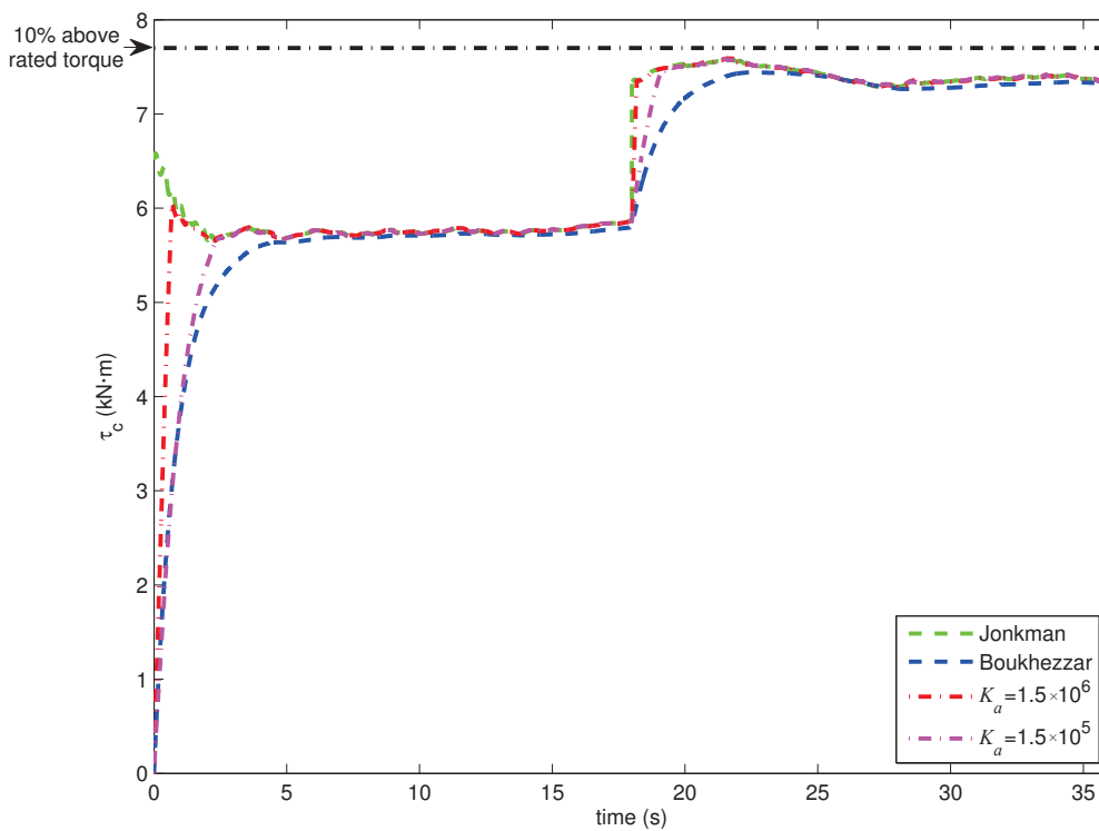
Figure 7. Torque control.
