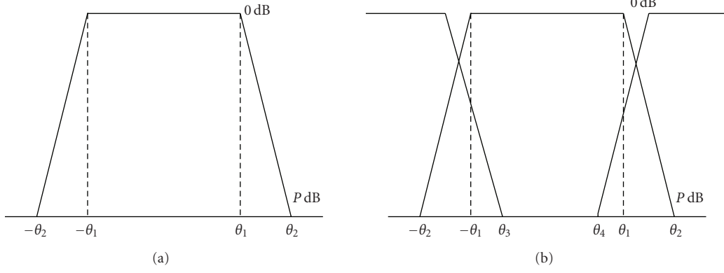
FIGURE 1: (a) Uplink/downlink antenna pattern model and (b) intersector interference model.
