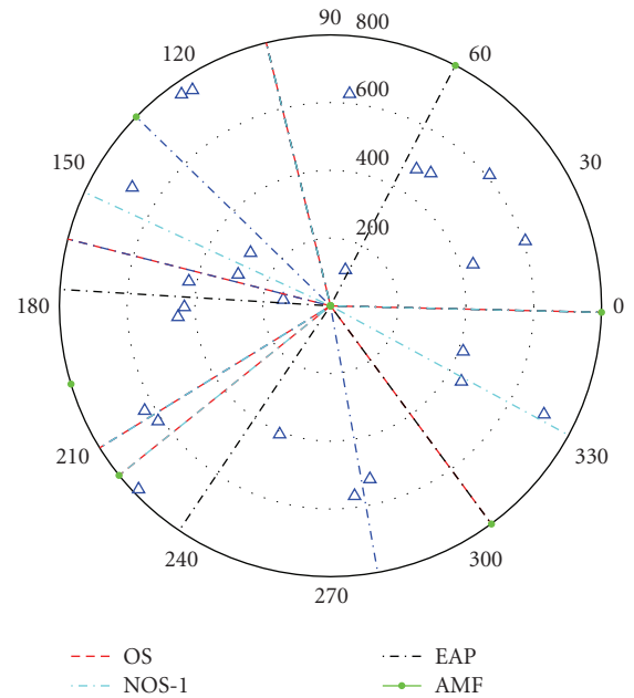
FIGURE 8: Sector boundaries for the downlink of a CDMA system with uniform user distribution. Number of users, M = 25 ; processing gain, N = 16 ; number of sectors, K = 6 .
