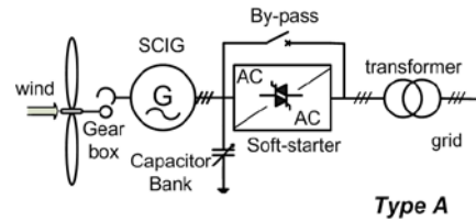
Fig. 5. Fixed speed wind turbine with directly grid connected squirrel-cage induction generator.
