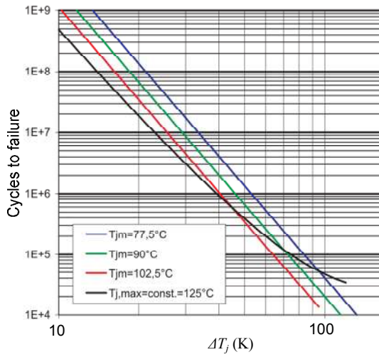
Fig. 12. Illustration of industrial standard cycles to failure vs. dT_j of IGBT module by Semikron [46].
