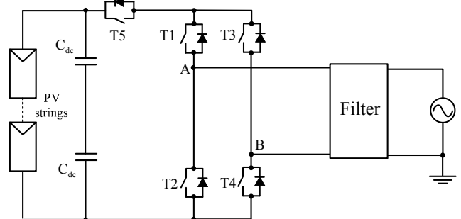
Fig. 6. H5 bridge topology for PV converter [37].
