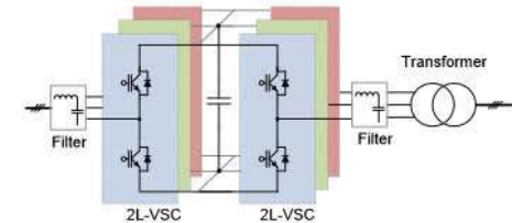
Fig. 9. Two-level back-to-back voltage source converter for wind turbines (2L-BTB)
