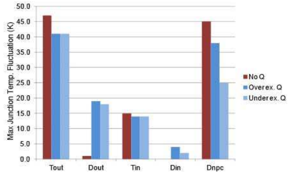
Fig. 23. Maximum thermal fluctuation of 3L-NPC inverter with different reactive powers (Considering parallel converters).
