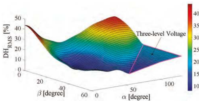
Figure 11. Amplitude trend of the distorting element ( DH_{RMS} ) versus \alpha and \beta .
