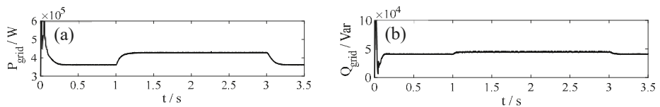
Figure 16. (a) active power of grid. (b) reactive power of grid.
