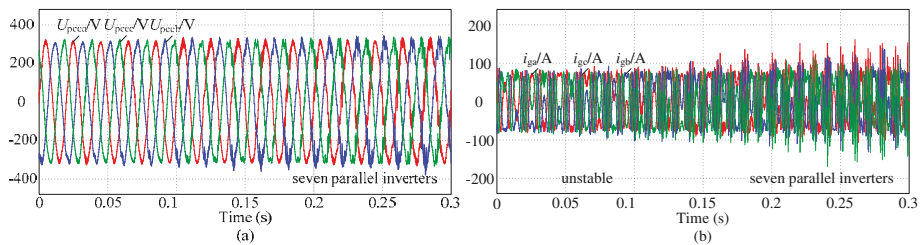
Figure 14. Simulation waveforms of PCC voltage u_{PCC} and the grid-connected current i_g in case I (seven parallel inverters). (a) PCC voltage u_{PCC} ; (b) grid-connected current i_g .
