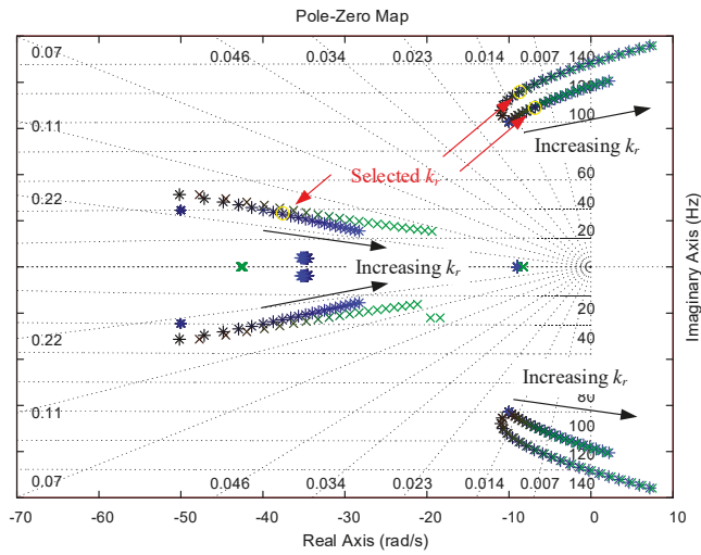
Figure 8. The impact of k_r (increased from 0 to 6.3) and the introduced current lowpass filters on the poles distribution of synchronverter system. Cross: poles without current lowpass filters. Asterisk: poles with current lowpass filters.
