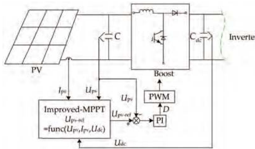
Figure 4. Overview of control scheme for pre-stage PV-Boost.
