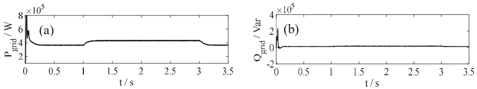
Figure 13. (a) active power of grid. (b) reactive power of grid.
