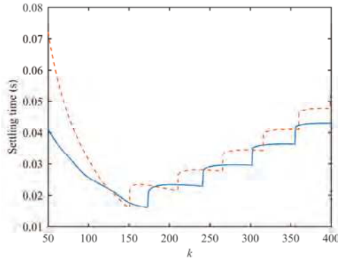
Figure 13. 2% settling time as a function of k .
