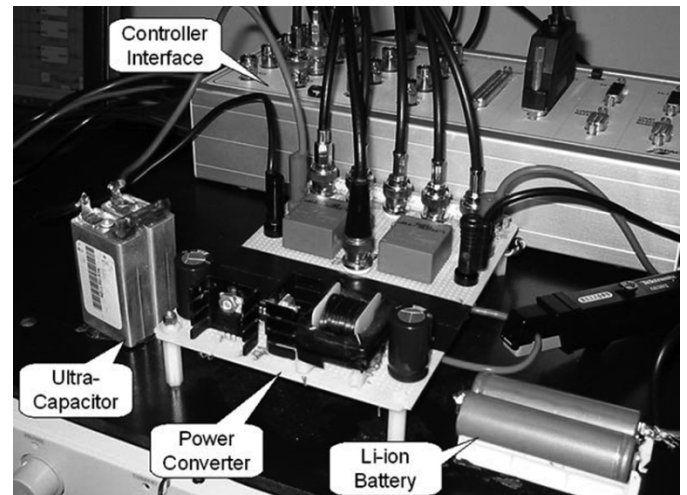
Fig. 5. Experimental setup of the active hybrid system.
