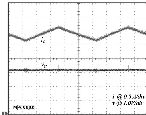
Fig. 13. Inductor current (0.5 A/div) and the converter output voltage (1 V/div) when the load demand is high.
