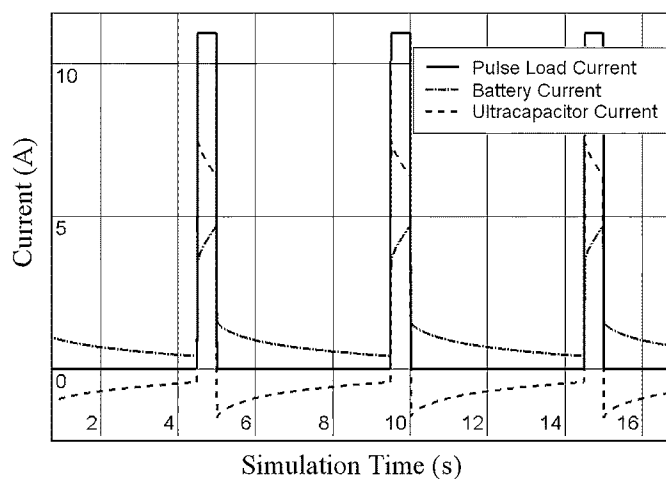
Fig. 14. Simulation results of the current waveforms of the passive hybrid.
