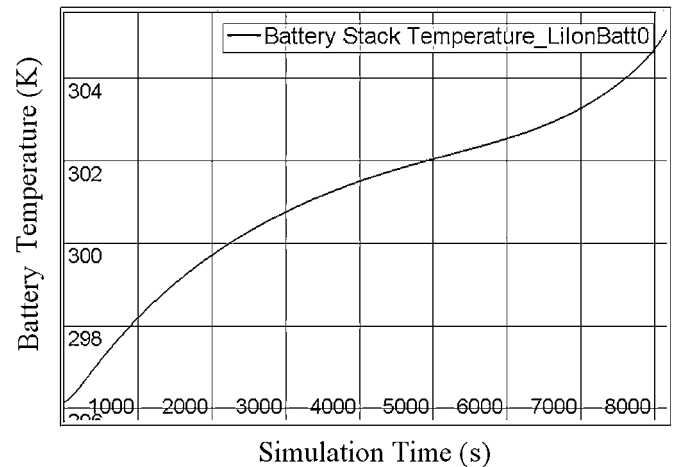
Fig. 20. Simulation result of the battery surface temperature of the active hybrid.
