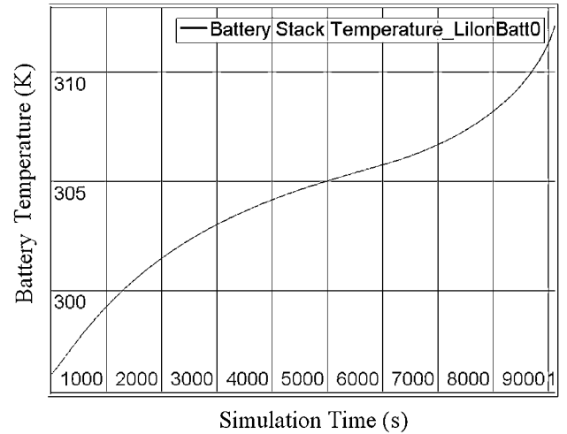
Fig. 19. Simulation result of the battery surface temperature of the passive hybrid.
