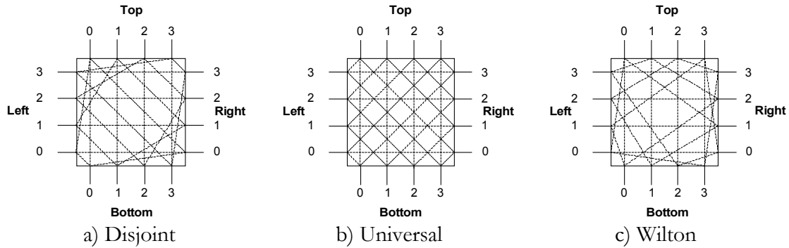
Figure 3.11 Three switch block topologies supported by VPR (from [46])
