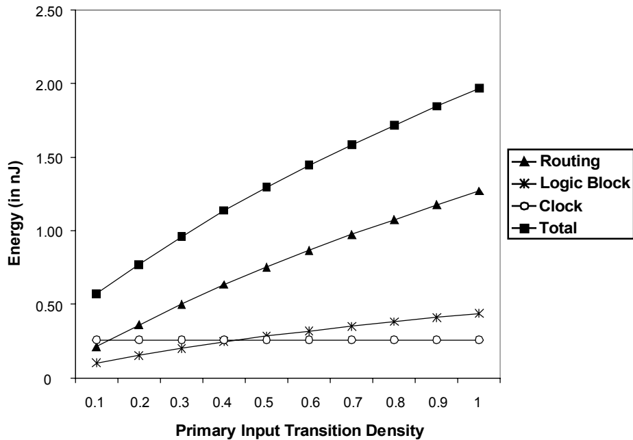
Figure 5.7 Energy versus primary input transition density
