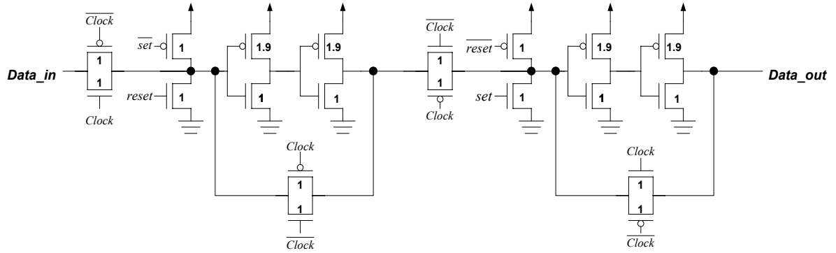
Figure 4.15 D-flip-flop with asynchronous set and reset
