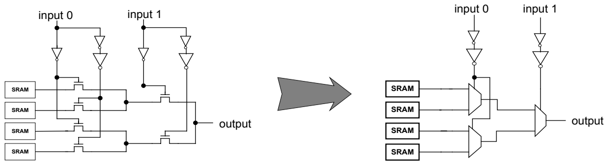
Figure 4.8 Modeling of a 2-Input look-up-table using 2-input multiplexers
