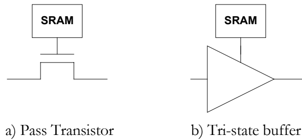
Figure 3.8 SRAM-controlled pass transistor and tri-state buffer
