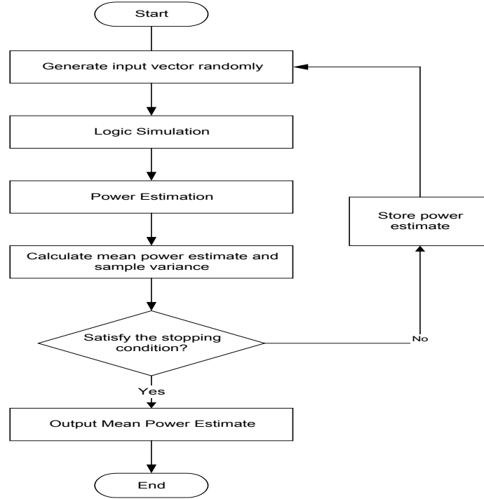
Figure 2.8 Monte Carlo power simulation
