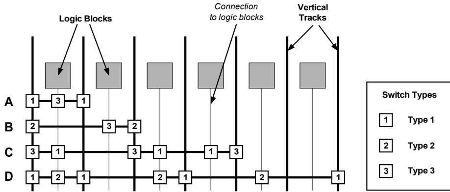
Figure 3.13 Wire segment examples
