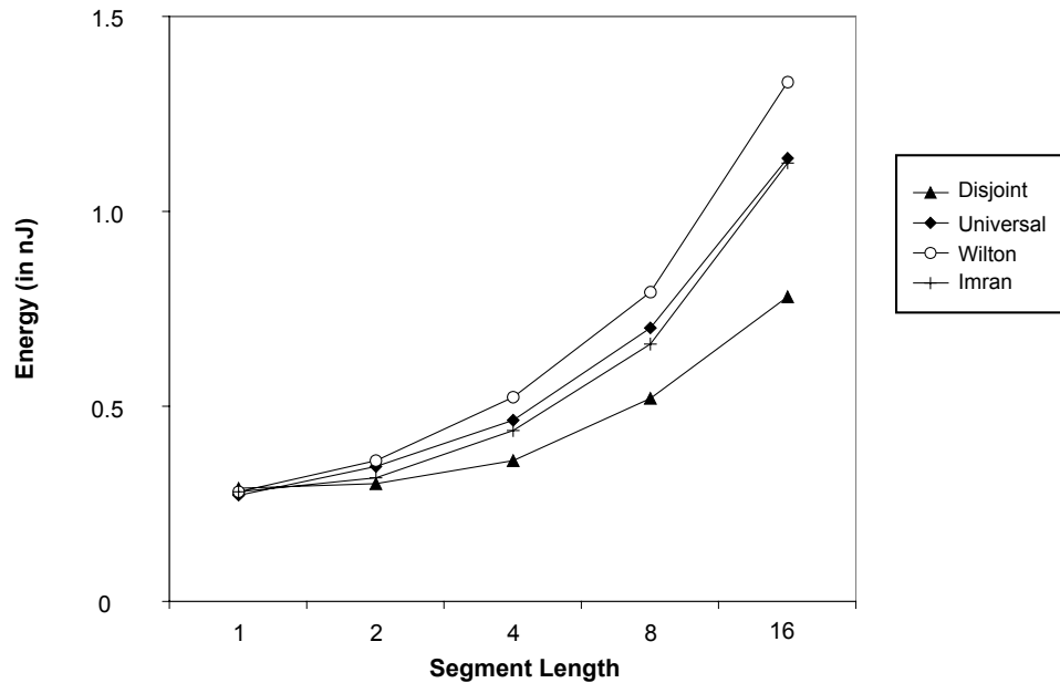
Figure 5.8 Energy versus segment length when input transition density is 0.2
