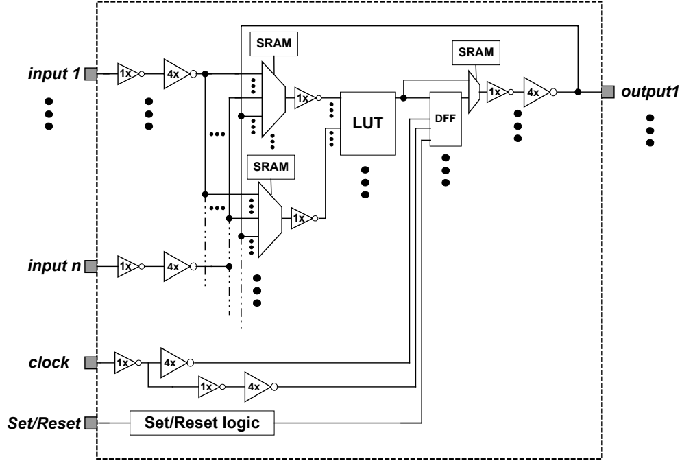
Figure 4.7 Schematic of a logic block (from [10])
