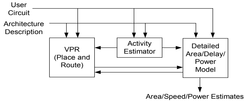
Figure 3.2 Framework with power model
