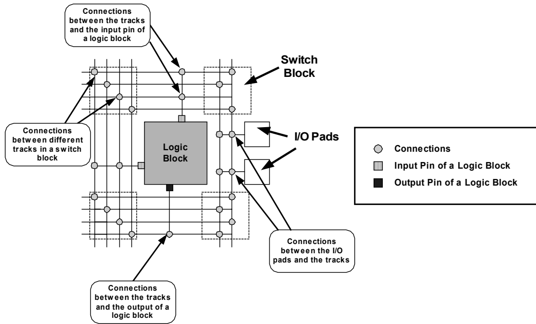
Figure 3.7 Connections between the logic blocks, routing tracks, and I/O pads
