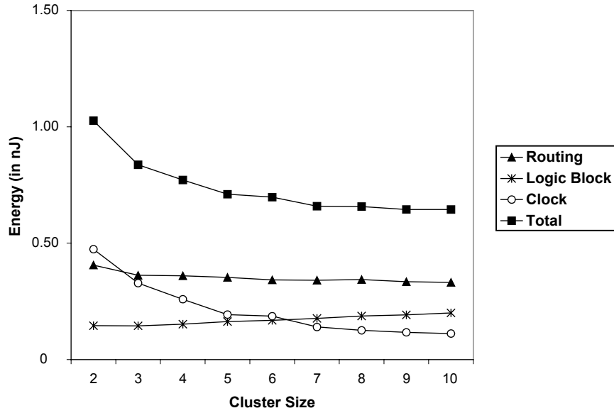
Figure 5.9 Energy versus cluster size when primary input transition density is 0.2
