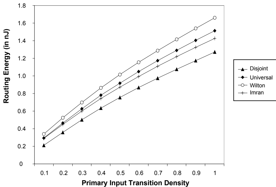
Figure 5.6 Routing energy versus primary input transition density
