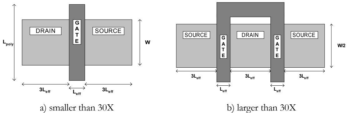
Figure 4.3 Layout of transistors
