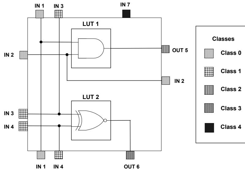
Figure 3.5 An example on logic block description
