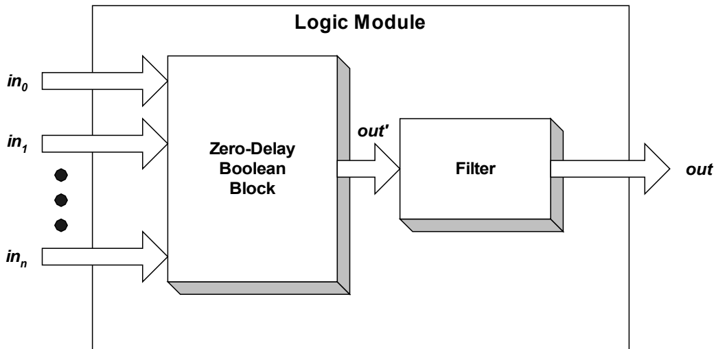
Figure A.1 Timing Model for Each Logic Module (from [50])
