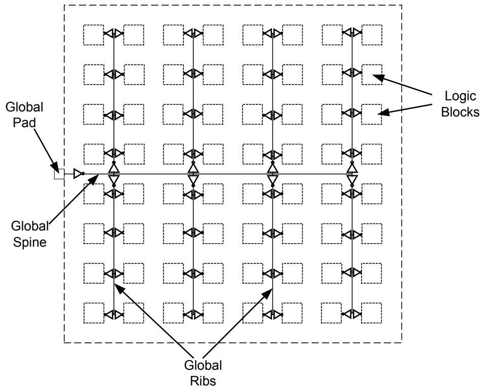
Figure 2.5 “Spines and Ribs” clock distribution network (from [2])
