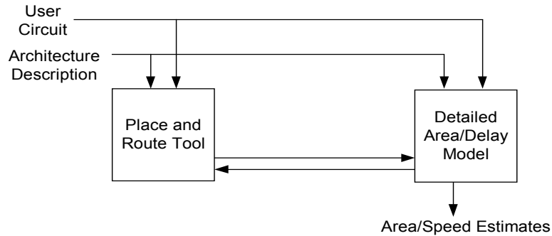
Figure 3.1 VPR framework
