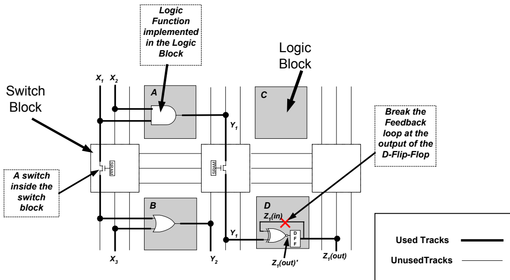
Figure 4.1 Logic functions implemented in the FPGA
