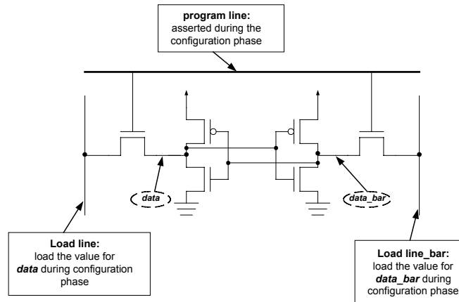
Figure 3.3 Schematic of a six-transistor SRAM cell
