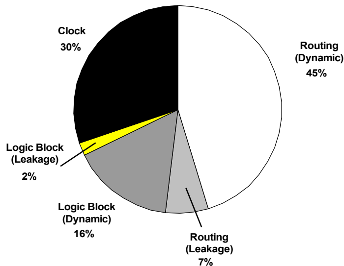
Figure 5.11 Energy distribution when primary input transition density is 0.2
