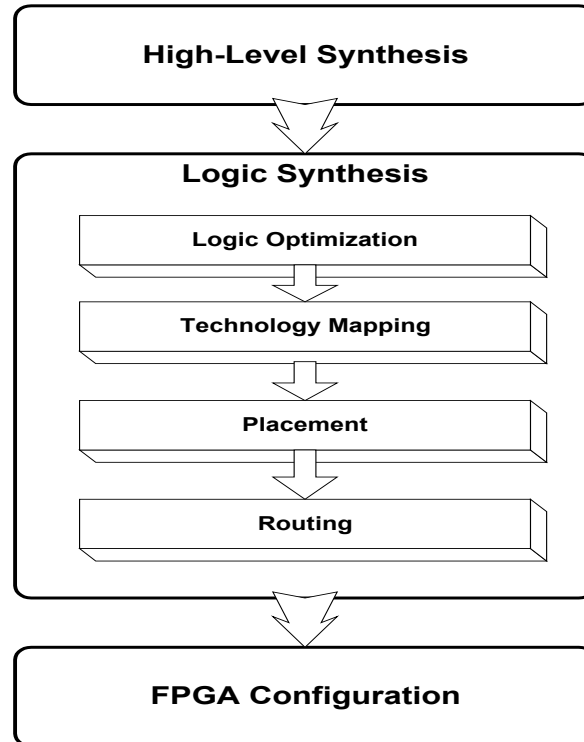
Figure 2.6 A typical FPGA CAD flow
