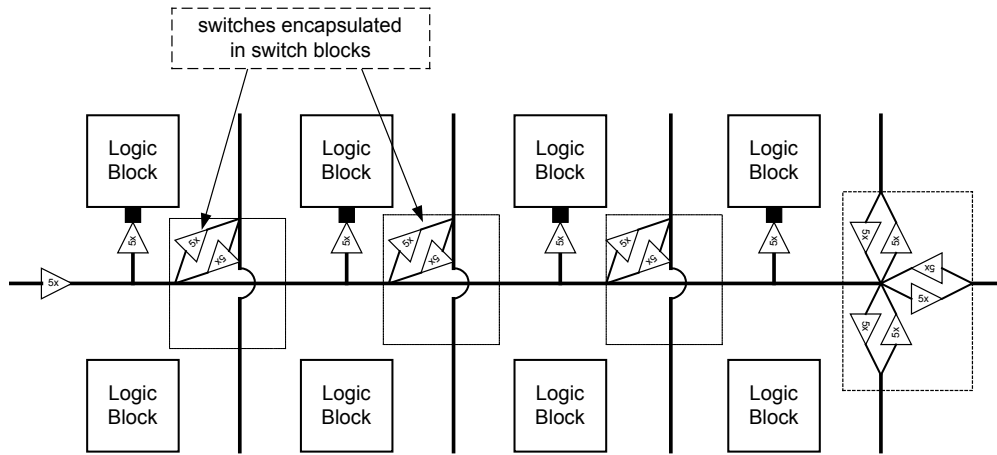
Figure 4.4 Wiring assumed for dynamic power experiment
