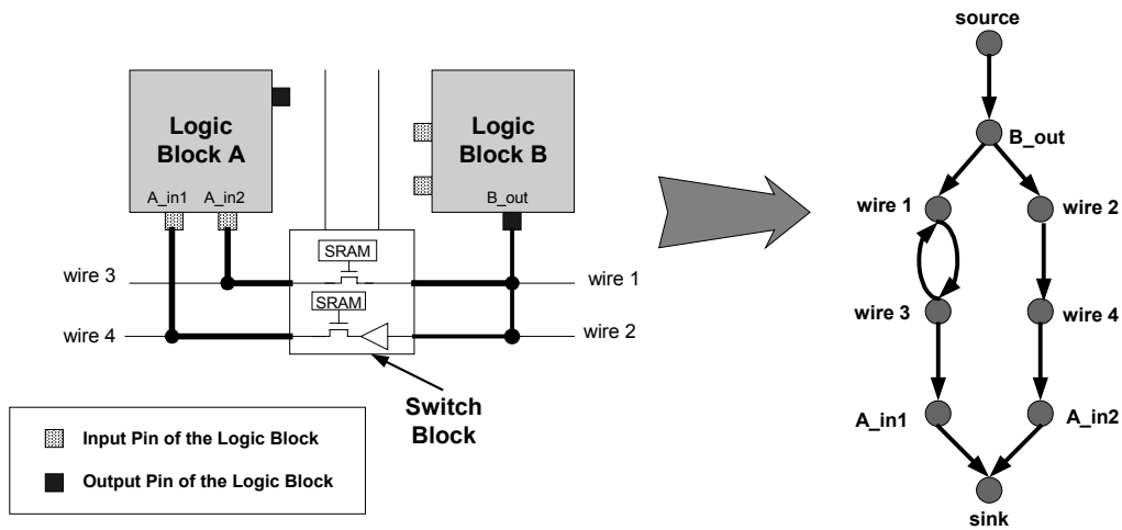
Figure 3.14 Routing resource graph for connections between two logic blocks
