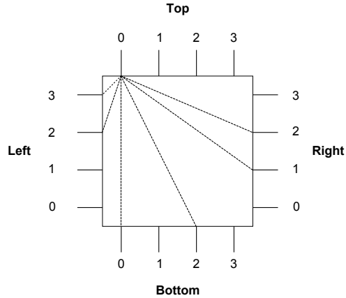
Figure 3.10 Switch block connection flexibility
