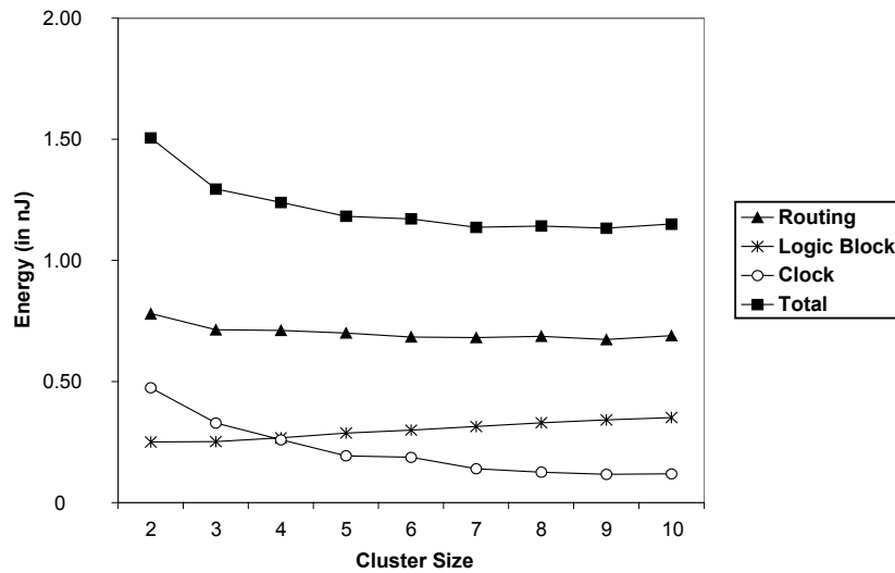
Figure 5.3 Energy versus cluster size
