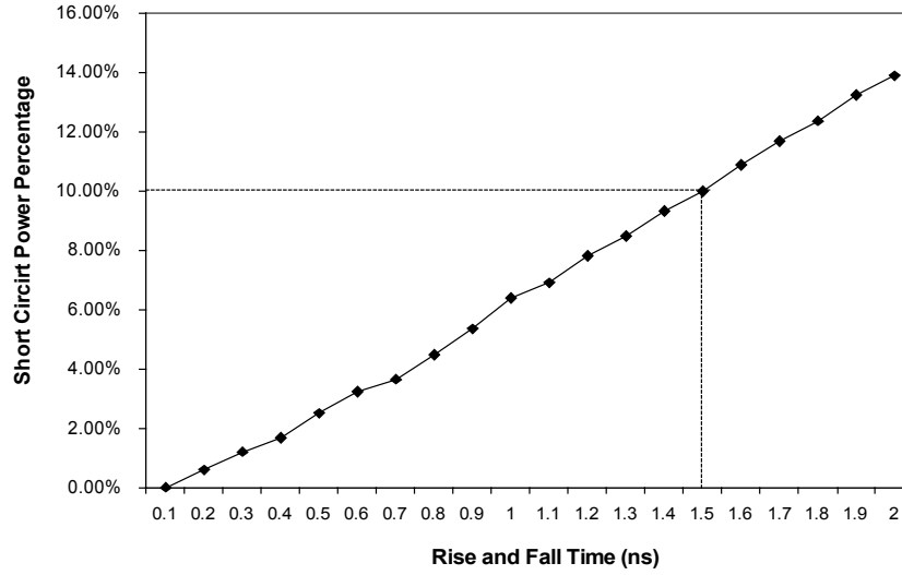
Figure 4.18 Short-circuit power percentage for one segment length
