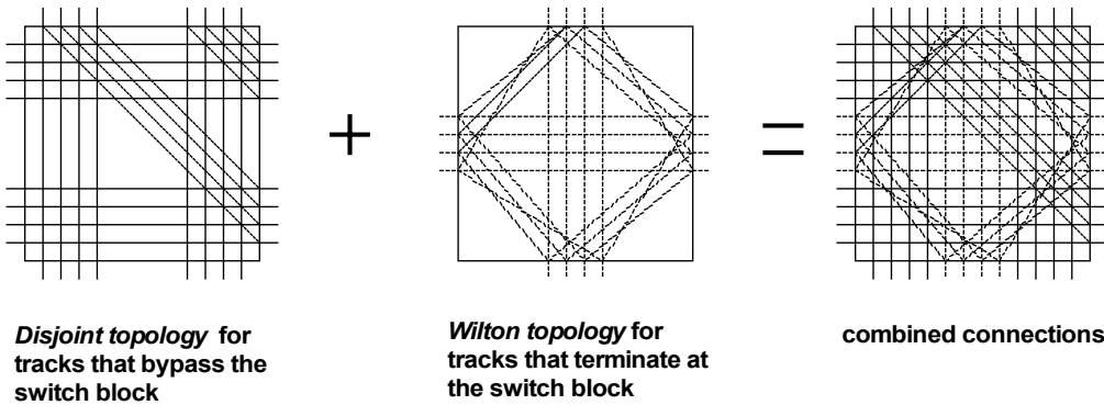
Figure 3.12 Imran switch block [46]
