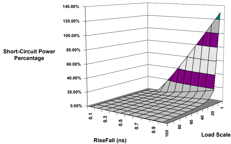
Figure 4.17 Short-circuit power percentage for the 1X inverter
