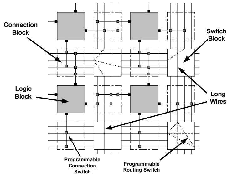
Figure 2.4 An island-style FPGA (from [10])
