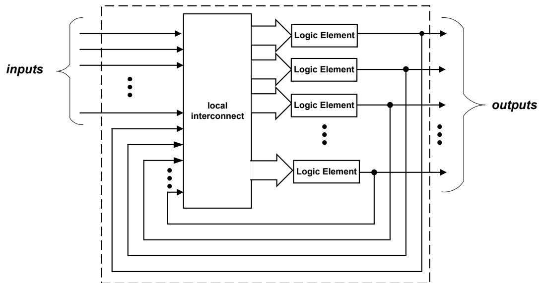
Figure 2.3 A hierarchical view of a logic block (from [10])
