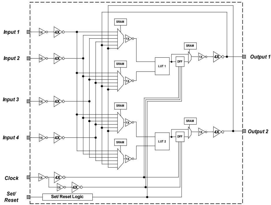
Figure 3.4 Schematic of a clustered logic block with 2 LUTs and 4 inputs
