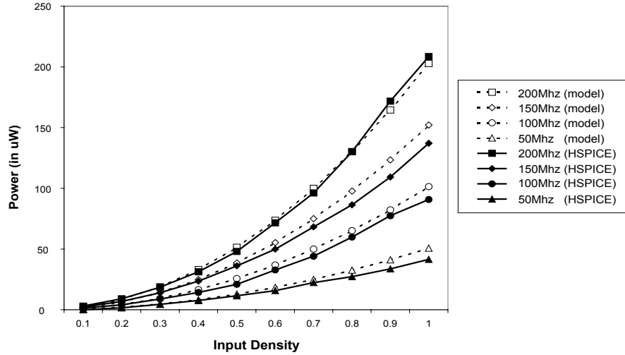
Figure 4.16 Dynamic power of D-flip-flop versus input density
