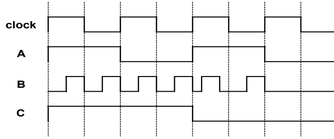
Figure 2.9 Examples of signals represented transition densities and static probabilities
