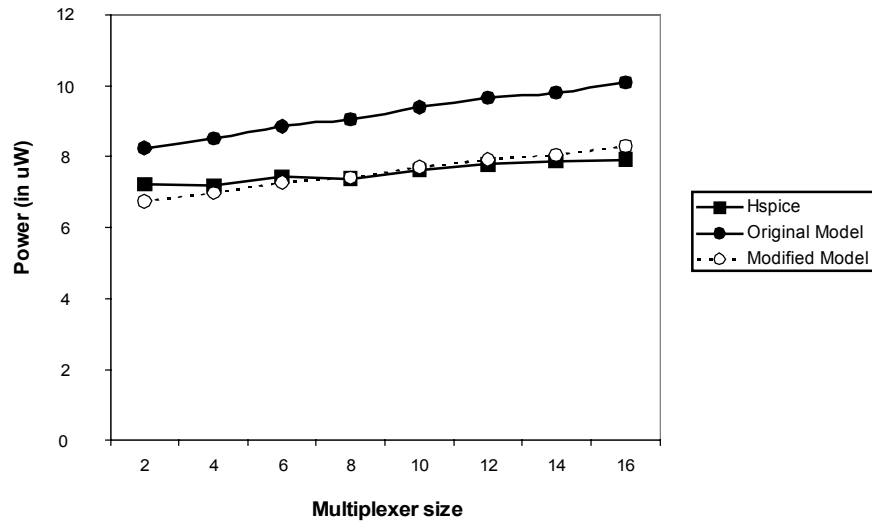
Figure 4.14 Power versus multiplexer size at an average input transition density of 0.5
