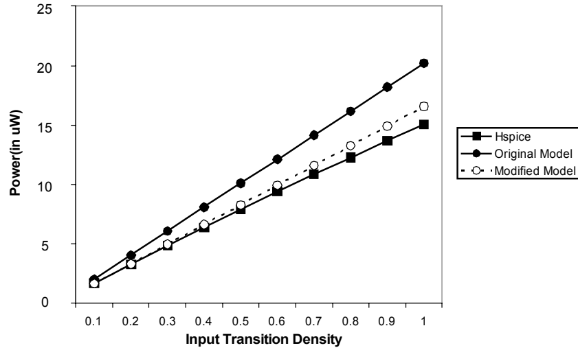
Figure 4.13 Power versus different average input transition densities for a 16-Input Multiplexer
