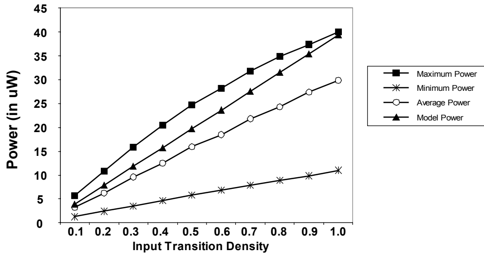
Figure 4.10 Power versus average input transition densities for a 4-Input LUT
