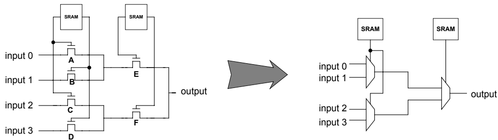
Figure 4.12 Modeling of a 4-input multiplexer using 2-input multiplexers
