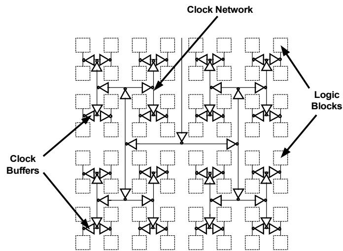
Figure 3.16 An H-Tree clock distribution network
