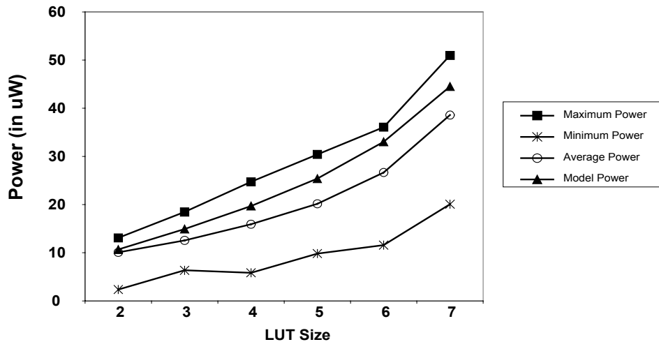
Figure 4.11 Power versus different LUT sizes with an input transition density of 0.5
