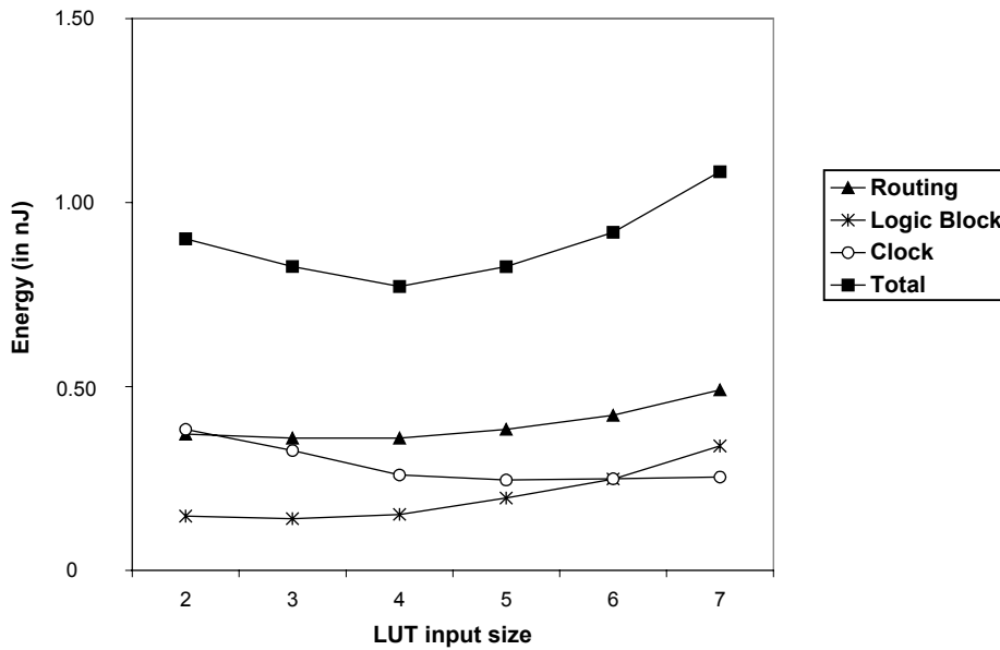
Figure 5.10 Energy versus look-up-table size when primary input transition density is 0.2
