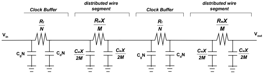
Figure 3.17 Distributed RC ladder network model for a long clock wire segment
