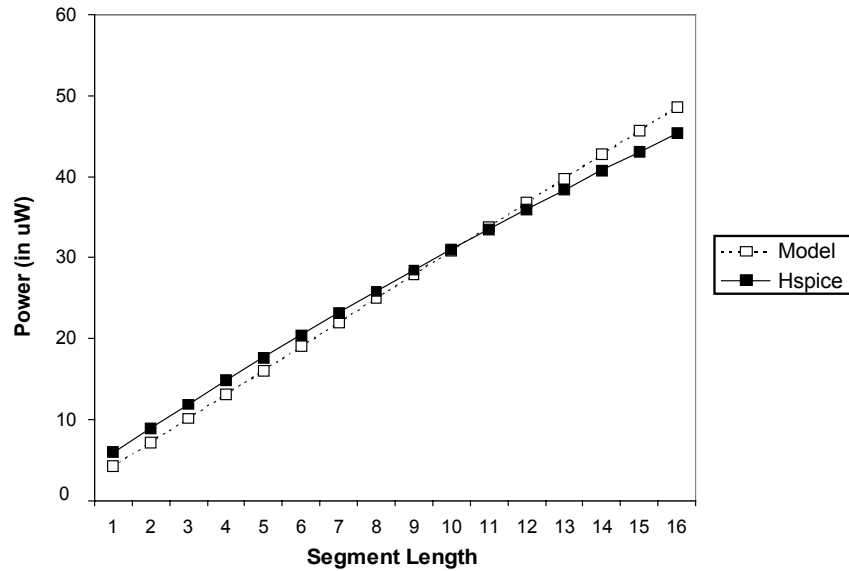
Figure 4.6 Dynamic power for a one segment at 20Mhz
