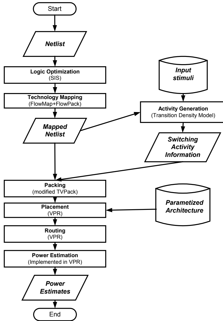
Figure 5.1 Power estimation flow for this project
