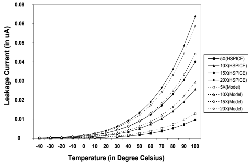
Figure 4.20 Leakage current versus temperature for different sizes of PMOS transistors
