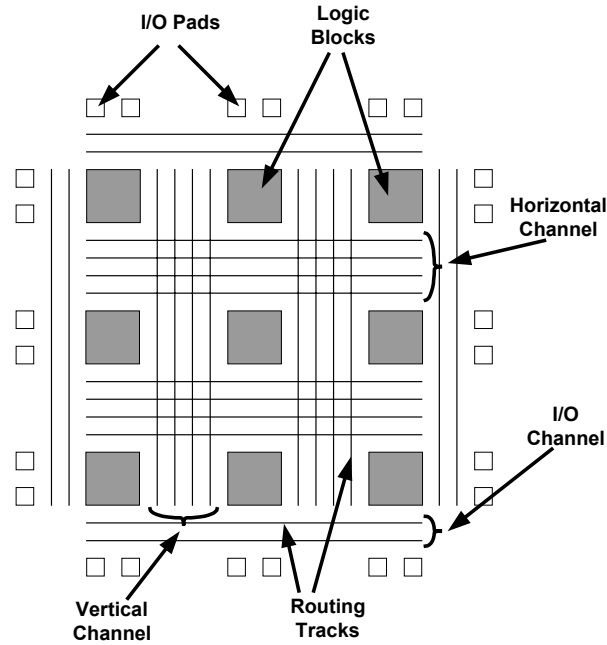
Figure 3.6 High-level FPGA model assumed by VPR
