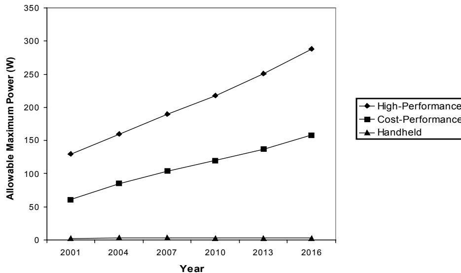
Figure 1.1 Projection of allowable maximum power for semi-conductor devices (from[30])
