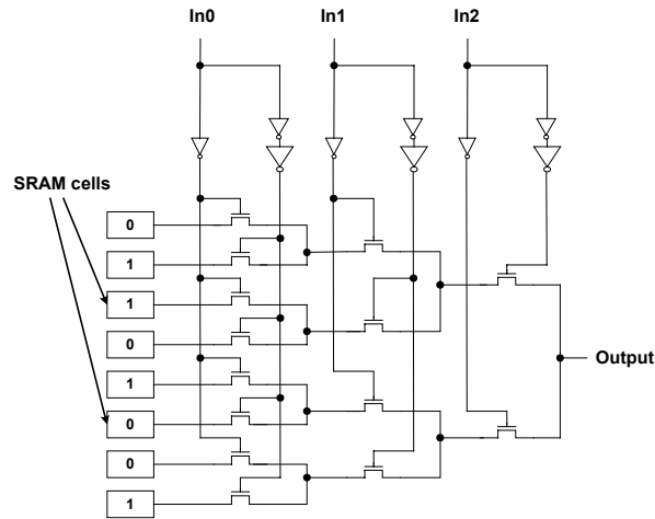
Figure 4.9 Example of worse case function for a 3-input LUT
