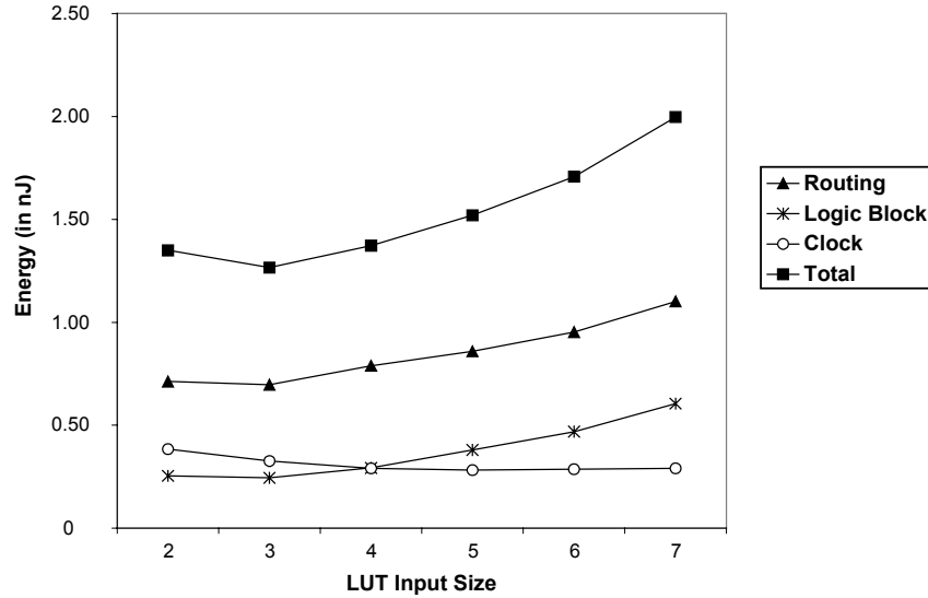
Figure 5.4 Energy versus look-up-table (LUT) size
