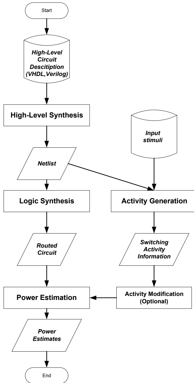
Figure 2.10 Power estimation flow
