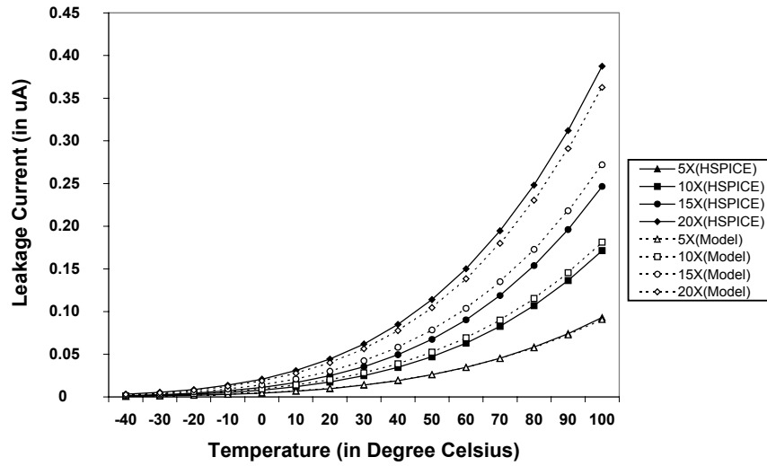
Figure 4.19 Leakage current versus temperature for different sizes of NMOS transistors
