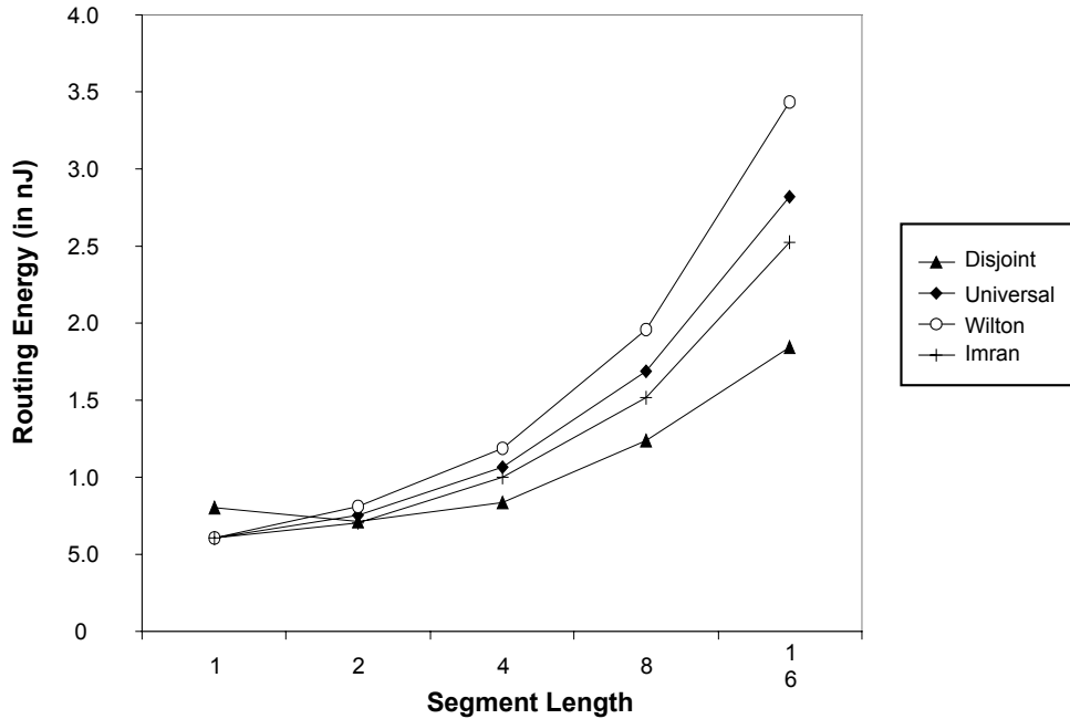
Figure 5.12 Routing energy versus segment length using breath-first algorithm
