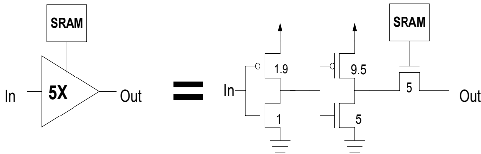
Figure 3.9 Schematic of a 5X tri-state buffer
