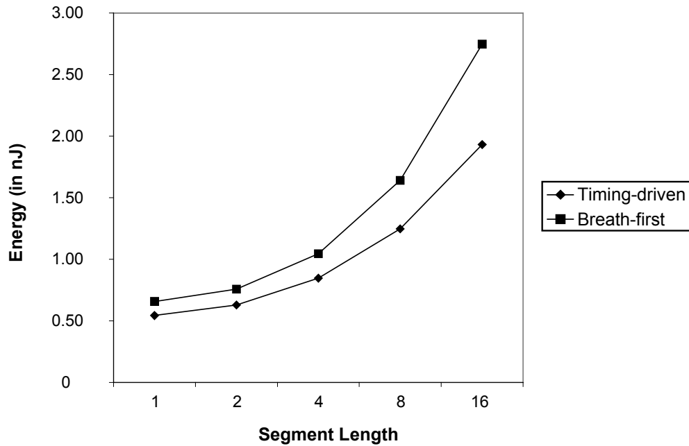
Figure 5.13 Average routing energy from timing-driven and breath-first algorithms
