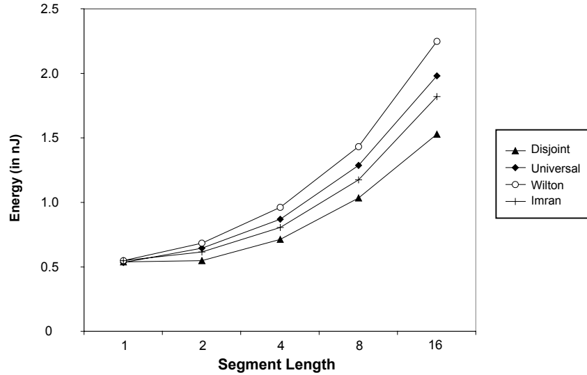
Figure 5.2 Energy vs. segment length
