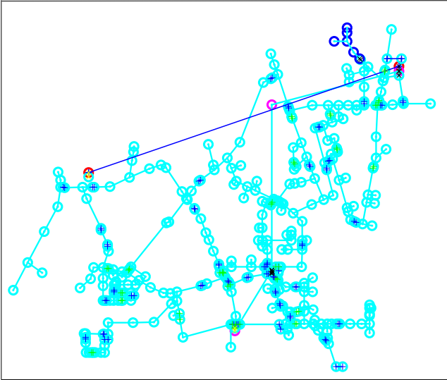
Fig. 1: A 396-node MV distribution network. Components: bus (circle), line branches (cyan line ending with ‘.’s), switches ( blue line ending with ‘+’s), transformers (black lines ending with ‘x’), open or out of service component (green dotted line); the node color representing its voltage levels: 115 kV (red), 34.5 kV(magenta), 12.47 kV(cyan), 4.80 kV(blue).
