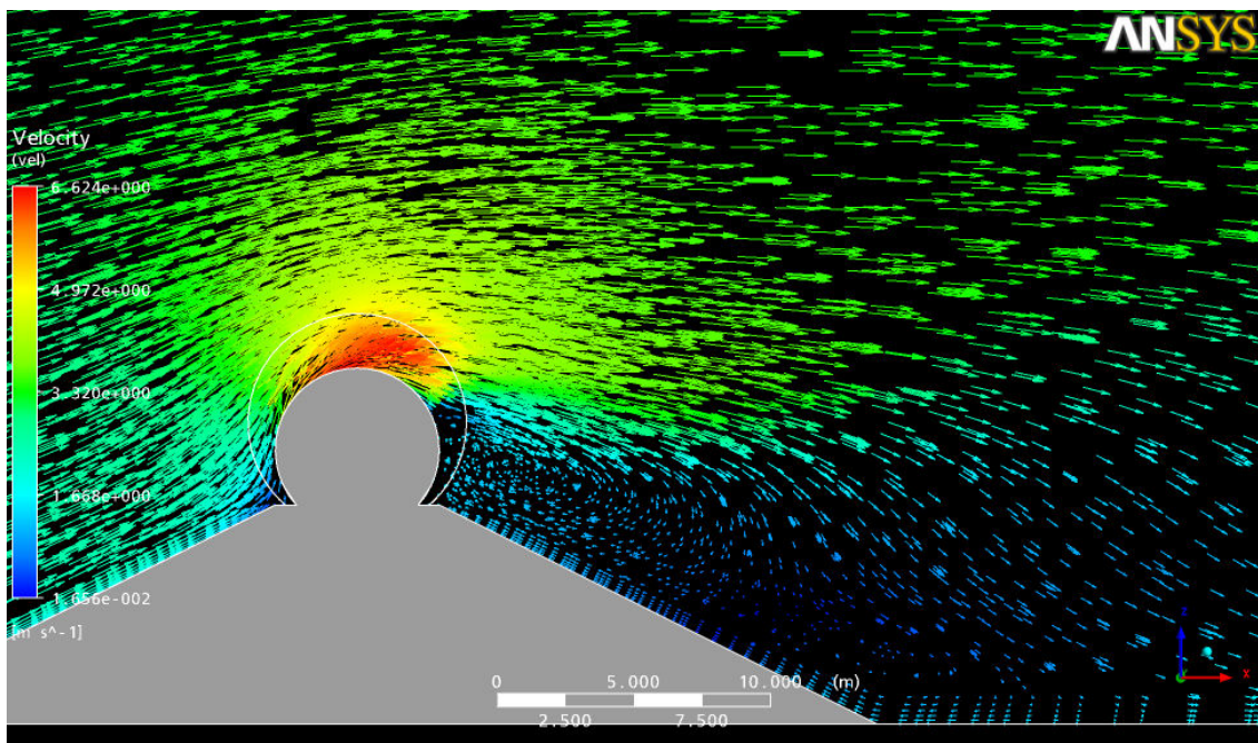
Fig 2.3 – The flow pattern in the case of no blades, representative of a steady state condition
