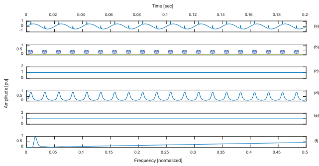
Fig. 6. (a) Multiple Spikes (b) frequency contour (c) amplitude-time curve (d) sum absolute values curve (e) phase curve (f) amplitude-frequency curve.
