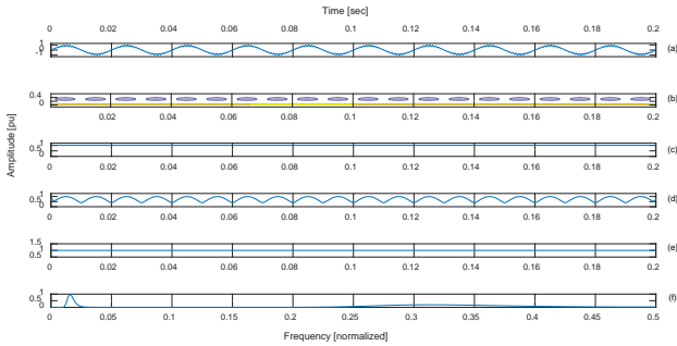
Fig. 2. (a) Flicker (b) frequency contour (c) amplitude-time curve (d) sum absolute values curve (e) phase curve (f) amplitude-frequency curve.
