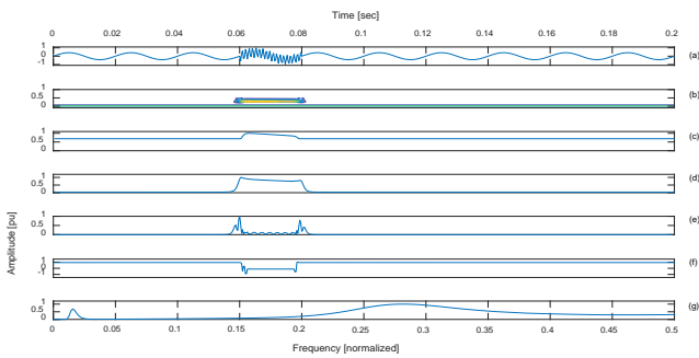
Fig. 3. (a) Oscillatory transient (b) frequency contour (c) amplitude-time curve (d) sum absolute values curve (e) second derivative of sum absolute values curve (f) phase curve (g) amplitude-frequency curve.
