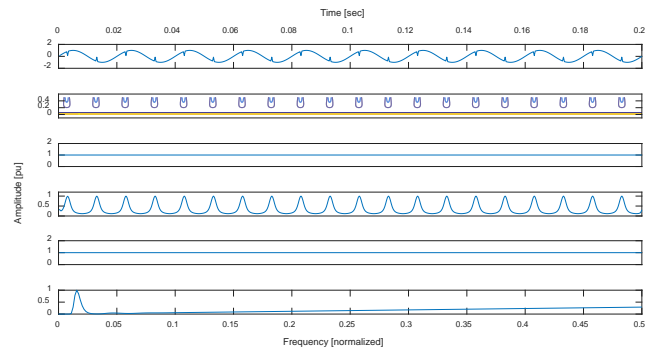
Fig. 5. (a) Multiple Notches (b) frequency contour (c) amplitude-time curve (d) sum absolute values curve (e) phase curve (f) amplitude-frequency curve.
