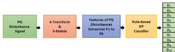
Fig. 1. Blok diagram of PQ disturbance by using rule-based decision tree.
