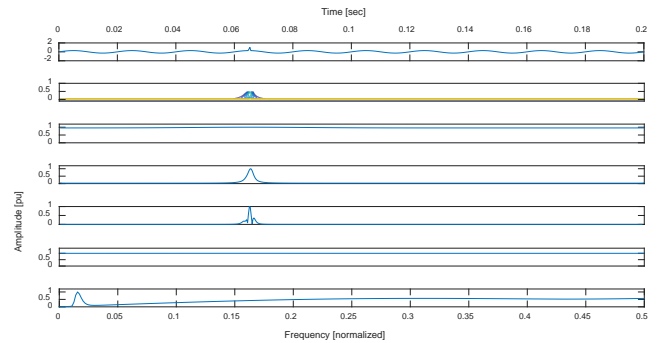
Fig.4. (a) Impulsive transient (b) frequency contour (c) amplitude-time curve (d) sum absolute values curve (e) second derivative of sum absolute values curve (f) phase curve (g) amplitude-frequency curve.
