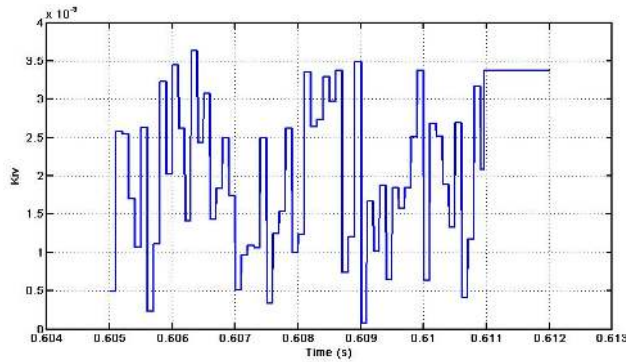
Fig. 11. Search process of K_{iv} when the system is islated
