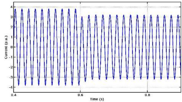
Fig. 13. System dynamic response at 0.6 seconds
