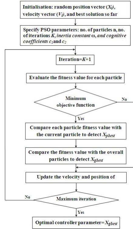
Fig. 5. Flowchart of the applied PSO algorithm
