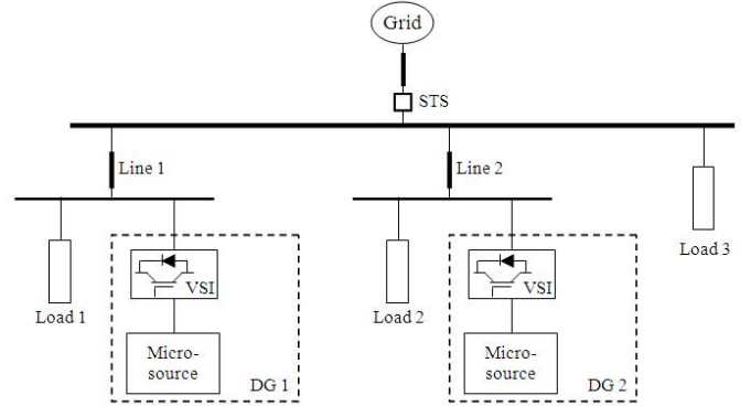
Fig. 1. An example of microgrid system
