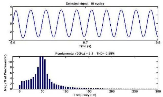
Fig. 14. Spectrum of the line current
