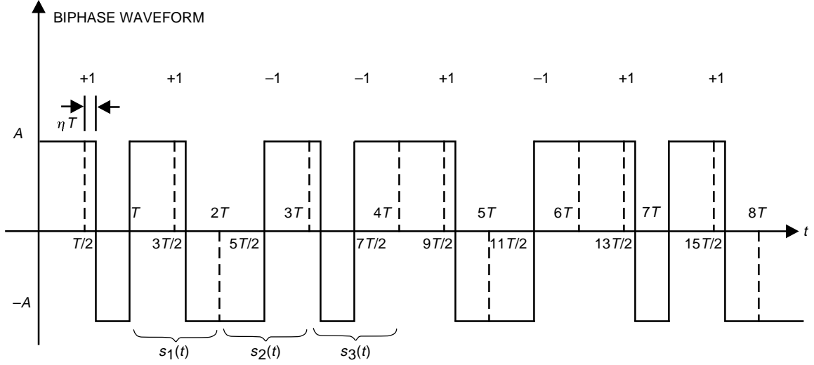
Fig. 2. An unbalanced, asymmetric biphas waveform for a typical data sequence.
