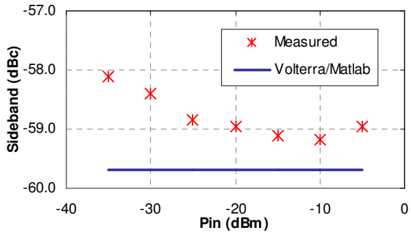
Fig. 10 Comparison of measured and calculated ripple sideband in decibels-below carrier.
