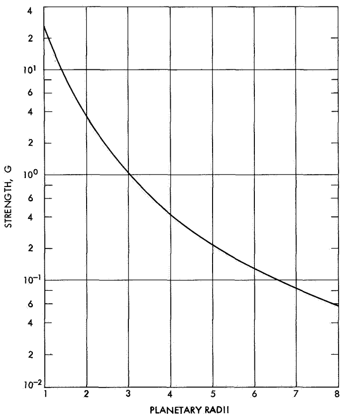
Fig. 36. Estimate of the Jupiter magnetic flux
