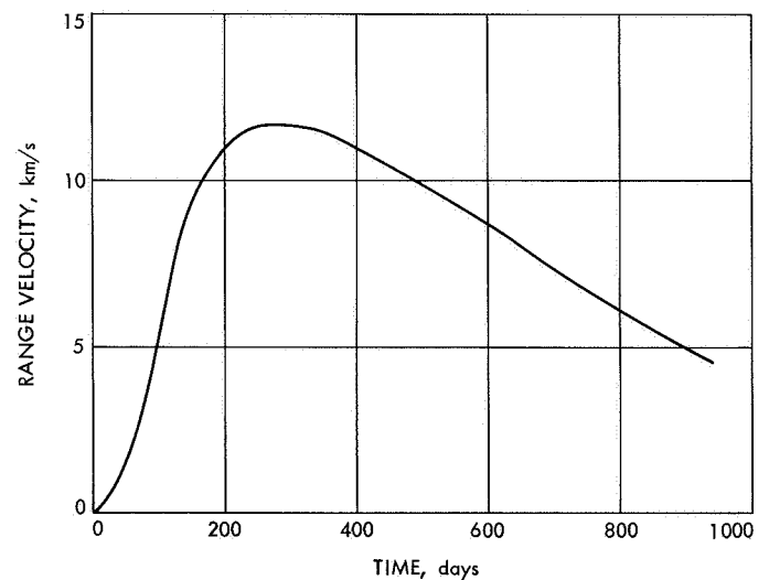
Fig. 31. Spacecraft velocity within the asteroid belt vs time
