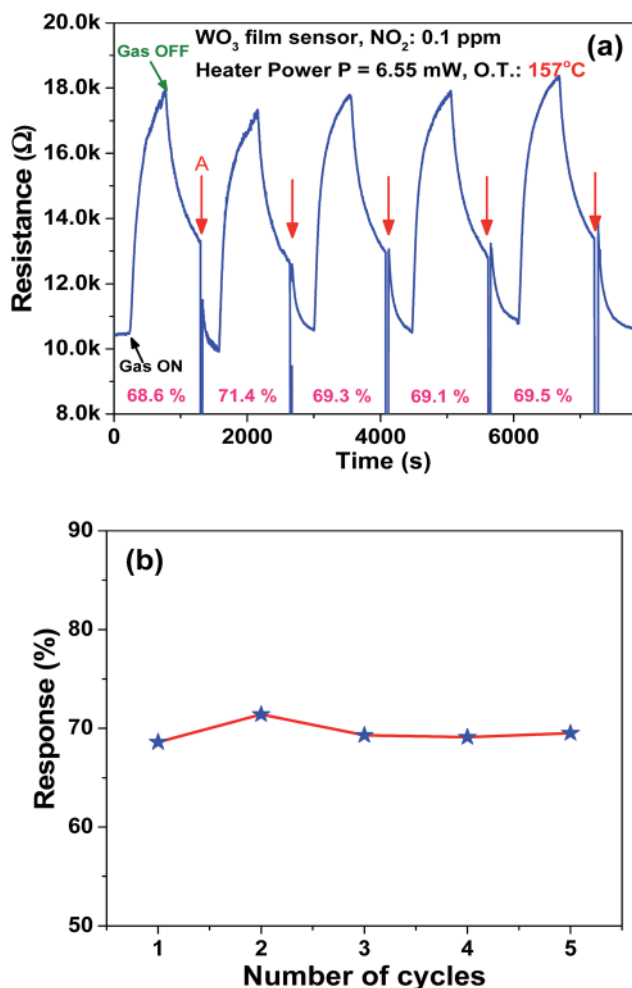
Fig. 9 (a) Sensor's repeatable response characteristics at a fixed operating temperature of 157^\circ\text{C} and gas concentration of 0.1 \text{ ppm} (symbol A indicates an abrupt decrease in resistance, resulting from a rapid increase in heater voltage) and (b) sensitivity versus number of cycles curve.
