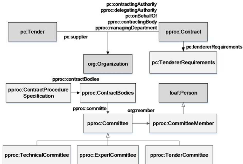
Figure 3. Parts-related classes
