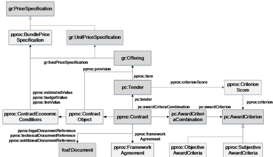
Figure 2. Contract object related classes
