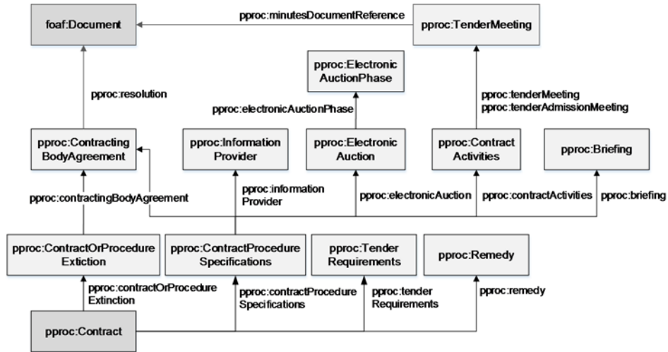
Figure 4. Procedure-related classes
