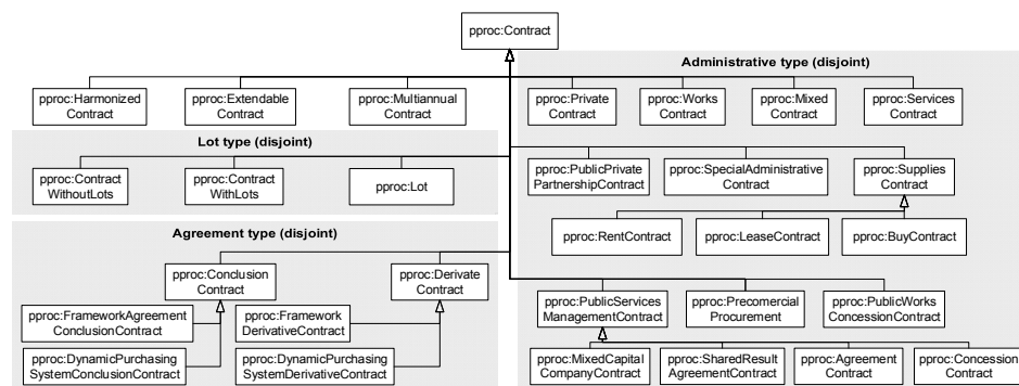
Figure 1. Classifications of the pproc:Contract class
