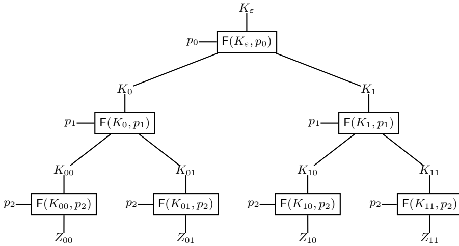
Fig. 3. Illustration of \Gamma^{F,m} for m = 2 . p_0, p_1 and p_2 are the random public values and K_\epsilon = K is the initial random key of the PRF. The output of the PRF for each X \in \{0, 1\}^2 is represented by Z_X , i.e., the leaves of the tree.
