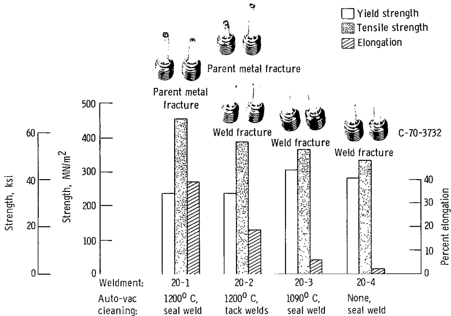
Figure 13. - Effect of auto-vac cleaning prior to diffusion welding AISI 1020 steel on room-temperature tensile properties. Welding parameters: temperature, 1090° C; pressure, 3.45x10 4 N/m 2 (5 psi) deadweight; time, 2 hours. All weldments were double normalized at 900° C after diffusion welding. Average of duplicate tests for each condition.
