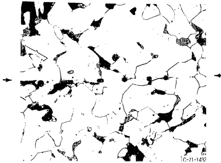
(c) Sealed weldment 20-3, auto-vac cleaned at 1090° C.
