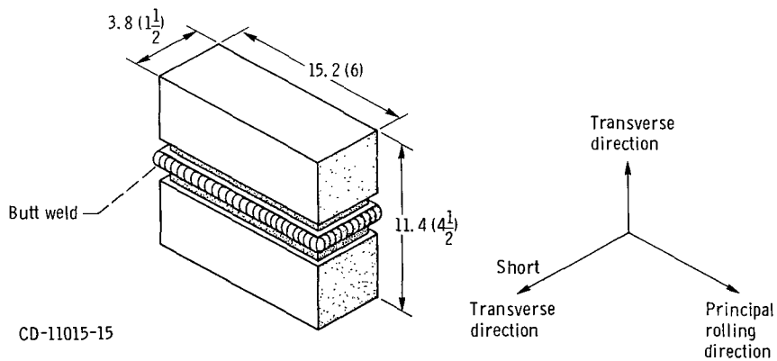
(b) 1090 o C and 980 o C weldments (numbers 20-1, 20-2, 20-3, 20-4, 18-1, 18-2, and 18-3).
