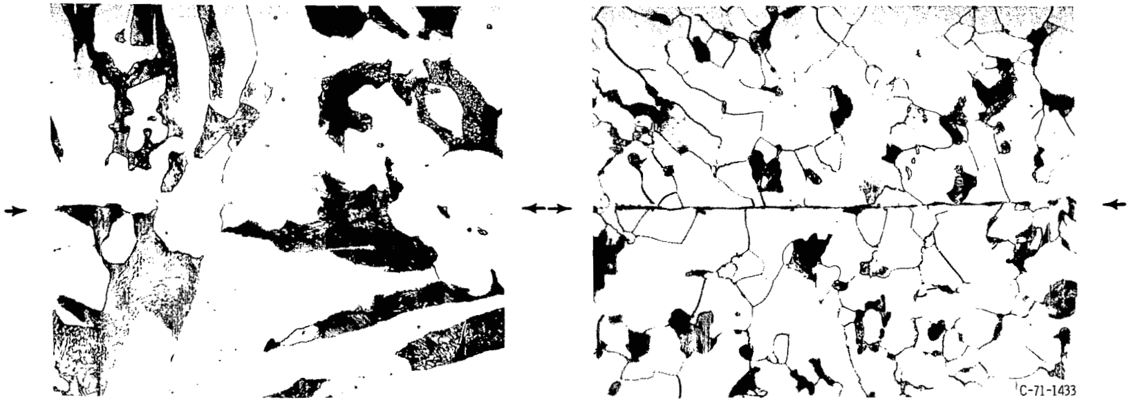
(a) Sealed weldment 18-1, auto-vac cleaned at 1200° C.
