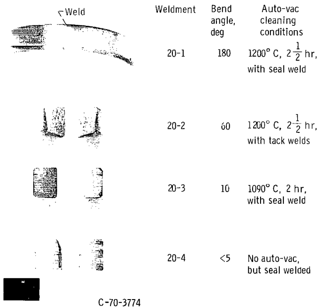
Figure 14. - Effect of auto-vac cleaning prior to diffusion welding AISI 1020 steel on bend properties. Diffusion weld parameters: temperature, 1090° C; pressure, 3.45x10 4 N/m 2 (5 psi); time, 2 hours. All weldments were double normalized at 900° C after diffusion welding.
