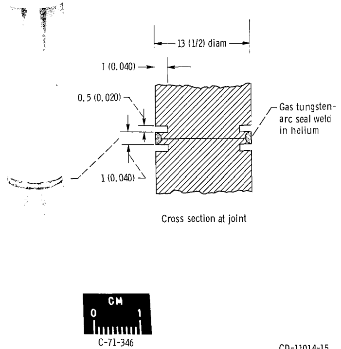
Figure 2. - Type 304 stainless steel assembly seal welded at periphery of faying surfaces. (Sketch illustrates joint design for seal weld. Dimensions are in mm (in.).)
