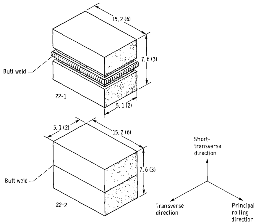
(a) 1200 o C weldments (numbers 22-1 and 22-2).
