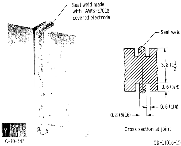
Figure 6. - Weld assembly in AISI 1020 steel with seal weld at periphery of faying surfaces. Cross-section sketch gives design of flange area at joint. (Dimensions are in cm (in. .))
