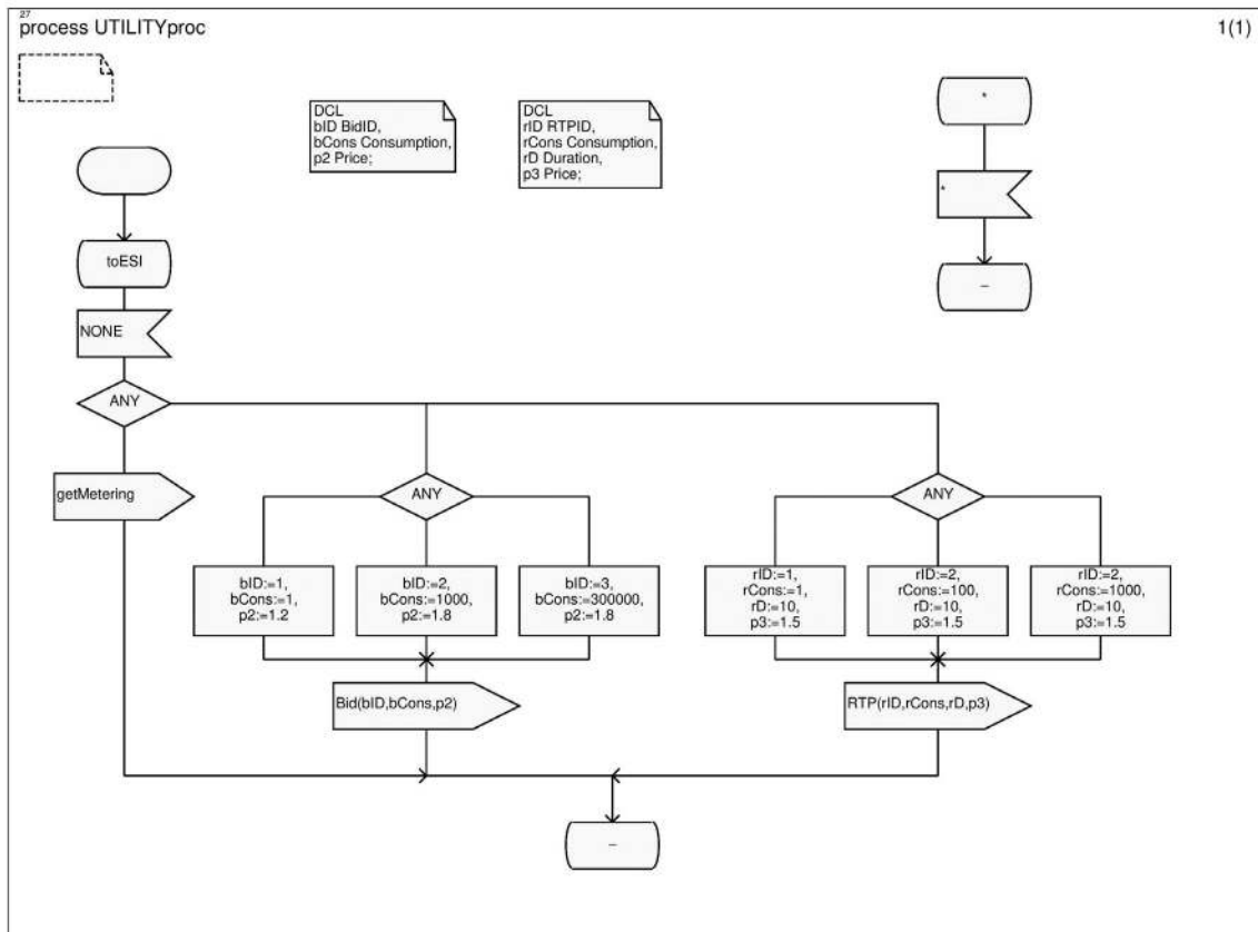
Figure 4. Process UTILITYproc.
