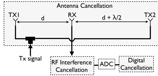
Figure 2: Block diagram of existing full duplex design with three cancellation techniques.
