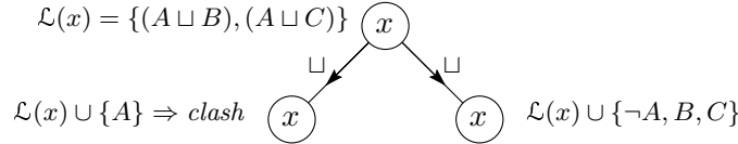
FIG. 7. Semantic branching search
