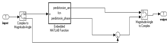
Fig.6. Pre-distorted system
