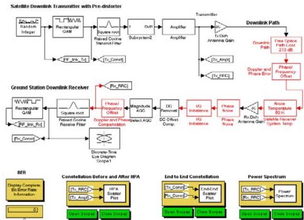
Fig.7. Simulink Model
