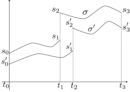
Figure 1: Graphical Distance between Executions.
