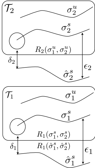
Figure 2: Illustration for Proof of Condition (D1)
