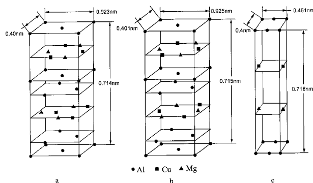
a Perlitz and Westgren model (from Ref. 17); b Mondolfo model (from Ref. 11); c Jin, Li and Yan model (from Ref. 19)
