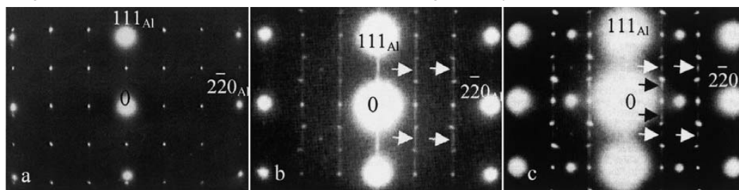
29 [\bar{1}\bar{1}2]_{Al} patterns and reflections from a \Omega (from Ref. 106); b \Omega (from Ref. 103) and c T_1 (from Ref. 107) (the superlattice spots are caused by \delta' phase)
