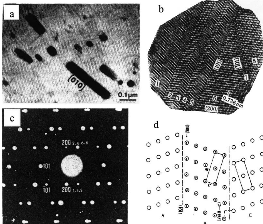
a bright field image; b high resolution image showing twin structure; c diffraction pattern corresponding to Fig. 4b; d illustration of glide reflection symmetry between neighbouring components of twins 4 Al_{20}Cu_2Mn_3 dispersoid phases in 2024 alloys (from Ref. 14)
