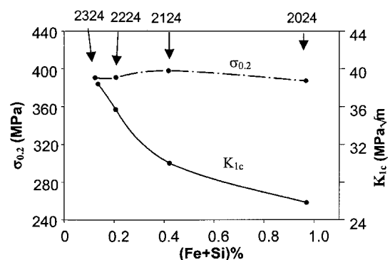
3 Effect of Fe and Si impurity contents on strength and fracture toughness of 2 \times 24 series alloys aged at 190°C for 12 h (from Ref. 5)
