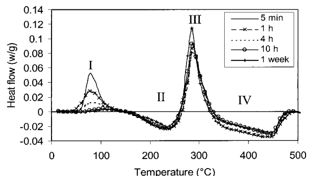
18 DSC thermograms of solution treated and quenched Al-2.81Cu-1.05Mg-0.41Mn (wt-%) alloy after aging for several intervals at 25°C; I, formation of clusters; II, dissolution of clusters and GPB2/S''; III, formation of S precipitates; IV, dissolution of S precipitates (from Ref. 31)
