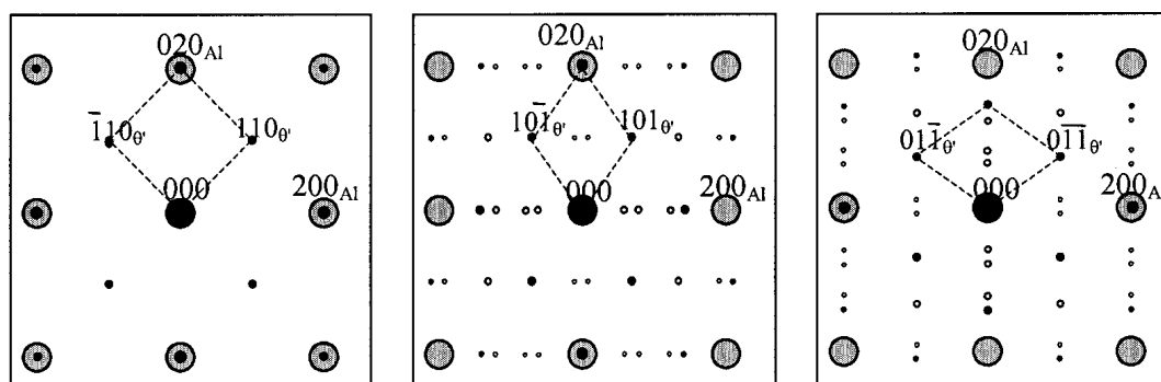
a [001]_{\theta'}/[001]_{\text{Al}} ; b [010]_{\theta'}/[001]_{\text{Al}} ; c [100]_{\theta'}/[001]_{\text{Al}}
