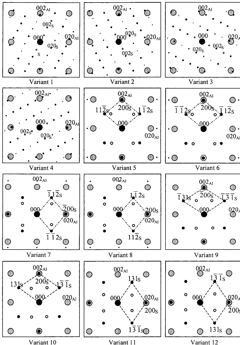
6 Simulated diffraction patterns of 12 variants of S phase observed from [100]_{Al} ; large grey circles present Al reflections, solid circles are S phase reflections and small open circles are double diffractions (based on Ref. 24 and software DiffraCt 1-2a )
