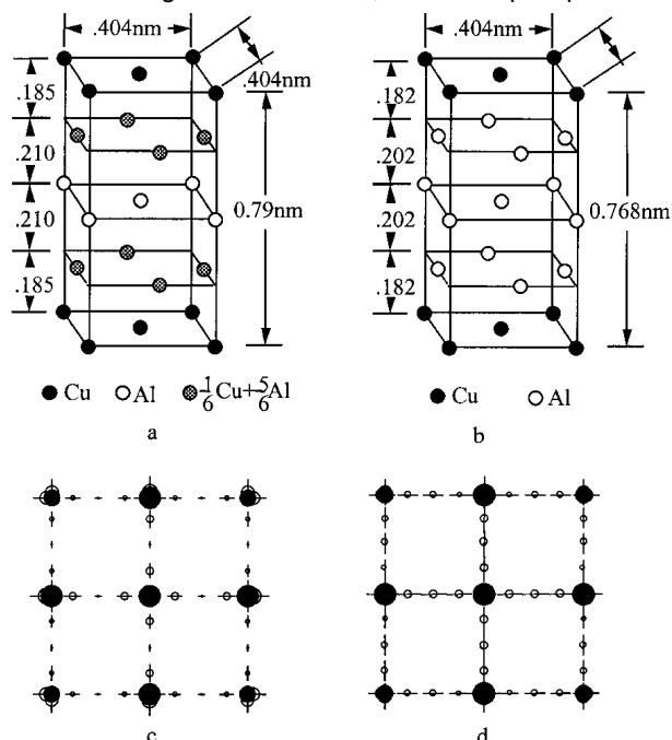
27 a Guinier model of GPII/ \theta'' (from Ref. 88); b Gerold model of GPII/ \theta'' (from Ref. 89), c simulated [001] Al diffraction patterns for Guinier model of GPII/ \theta'' and d simulated [001] Al diffraction patterns for Gerold model of GPII/ \theta'' ; simulation was carried out with Diffrac 1-2a software; sizes represent reflection intensities, and open and full circles correspond to GPII/ \theta'' and Al matrix, respectively
