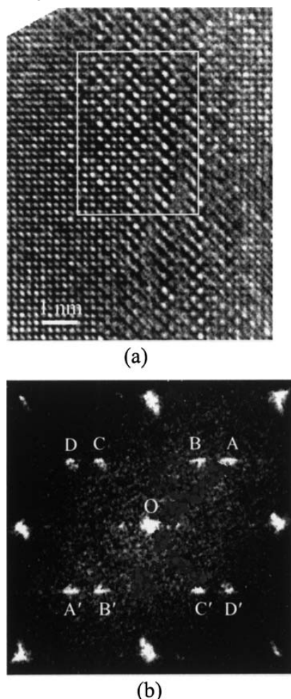
11 a HREM micrograph; b FT from frame shown in a 11 HREM micrograph and Fourier transformation in [100]_{Al} of Al-2.03Cu-1.28Mg (wt-%) alloy aged at 200°C for 4 h (adapted from Ref. 36, by courtesy of Professor A. Charai)
