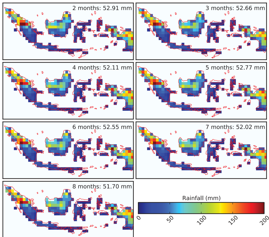
Figure 10. 1997 mean corrected GPCP rainfall rates (per month) during dry season based on using different time frames to convert GPCP to TRMM. The numbers indicate the 1997 mean rainfall for Indonesia during the dry season.
