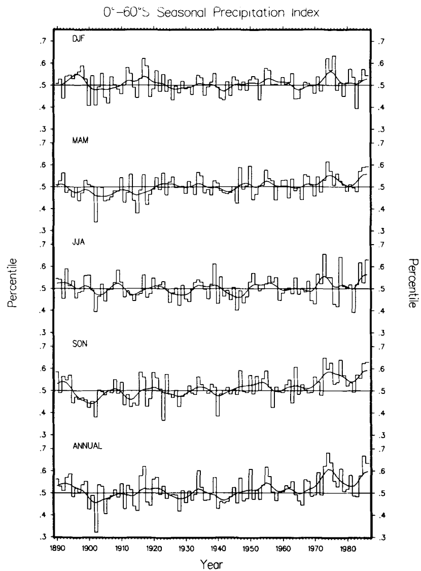
Fig. 11. Seasonal and annual precipitation index (mean of percentiles of the gamma probability distribution at all valid grid points) for the southern hemisphere for the period 1890–1986. The first year in which 50% of the maximum available number of grid points was present is 1890, compared with 1881 for the northern hemisphere.
