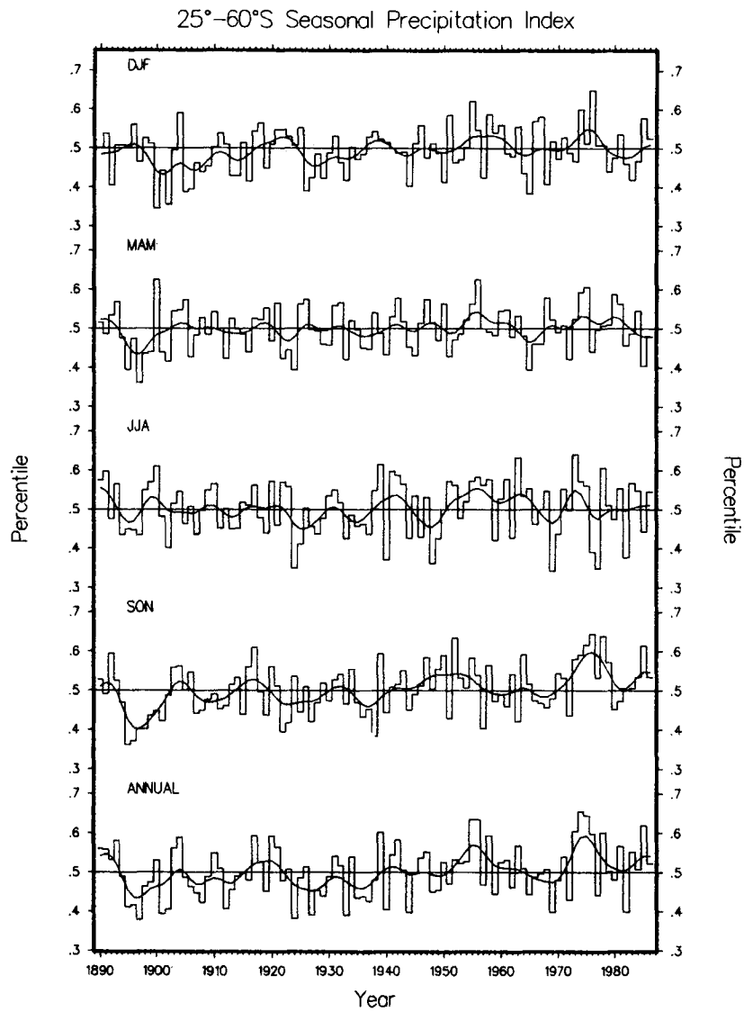
Fig. 9. As in Figure 3, except for the zonal belt 25°-60°S. This is referred to in the text as the southern temperate region.
