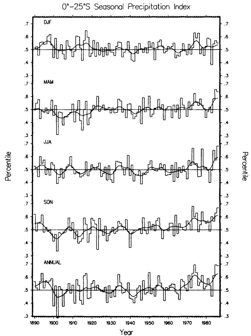
Fig. 10. As in Figure 3, except for the zonal belt 0°-25°S, referred to in the text as the southern tropical region.
