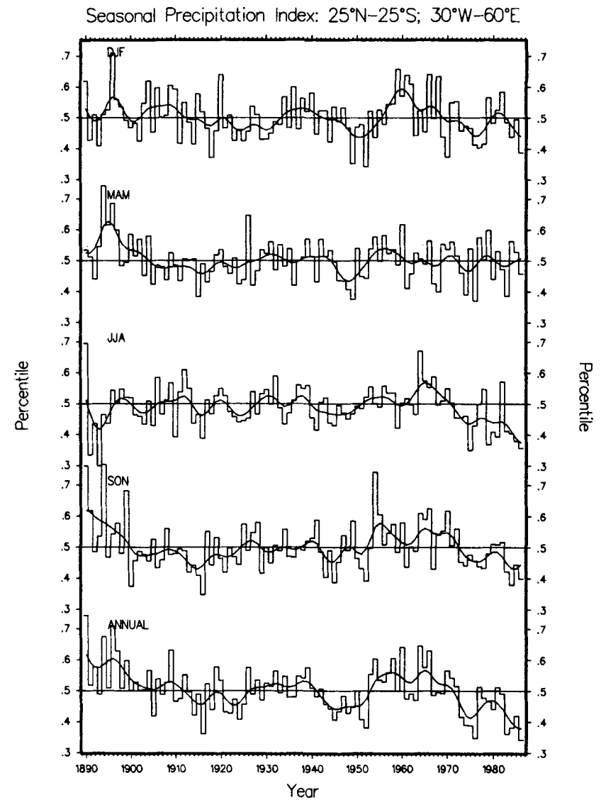
Fig. 8. As in Figure 3, except for the area 25°N–25°S, 30°W–60°E, referred to in the text as the southern Africa sector.
