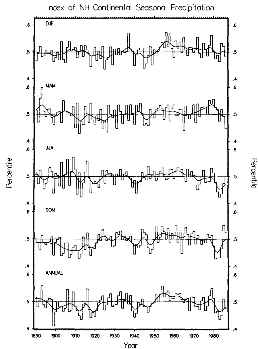
Fig. 12. As in Figure 11, except for the northern hemisphere land areas.
