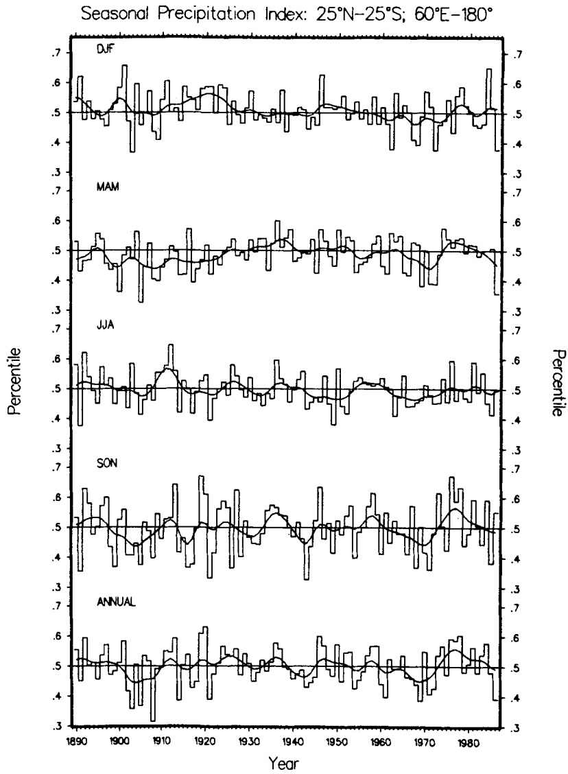
Fig. 7. As in Figure 3, except for the area 25°N–25°S, 60°E–180°E, referred to in the text as the Australasian sector.
