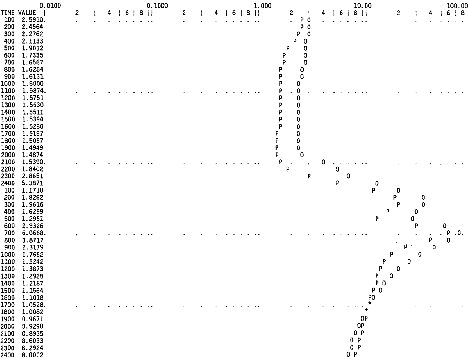
Figure 31.--Stormflow hydrograph plot.
