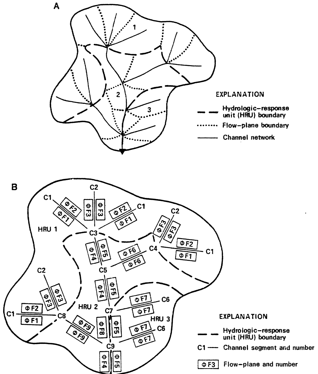
Figure 19.--Delineation of sample watershed: (A) Hydrologic response unit (HRU), flow-plane boundaries, and channel network; (B) schematic of flow planes and channel segments.
