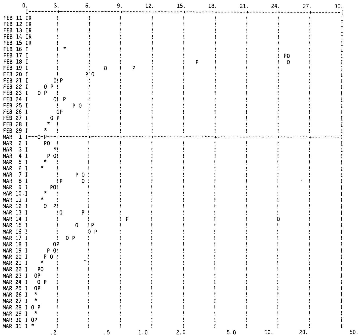
Figure 29.--Linear plot of mean daily discharge.
