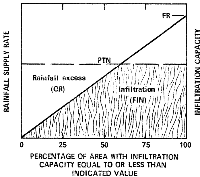
Figure 7.--The relation that determines rainfall excess (QR) as a function of maximum infiltration capacity (FR) and supply rate of rainfall (PTN).
