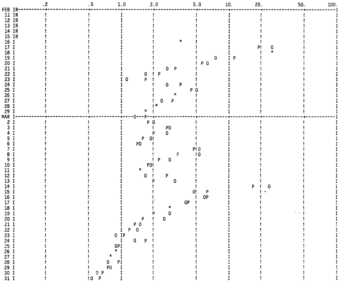
Figure II-6.--Line printer plot of simulated and observed daily mean discharge for Cane Branch watershed, February and March, 1956.
