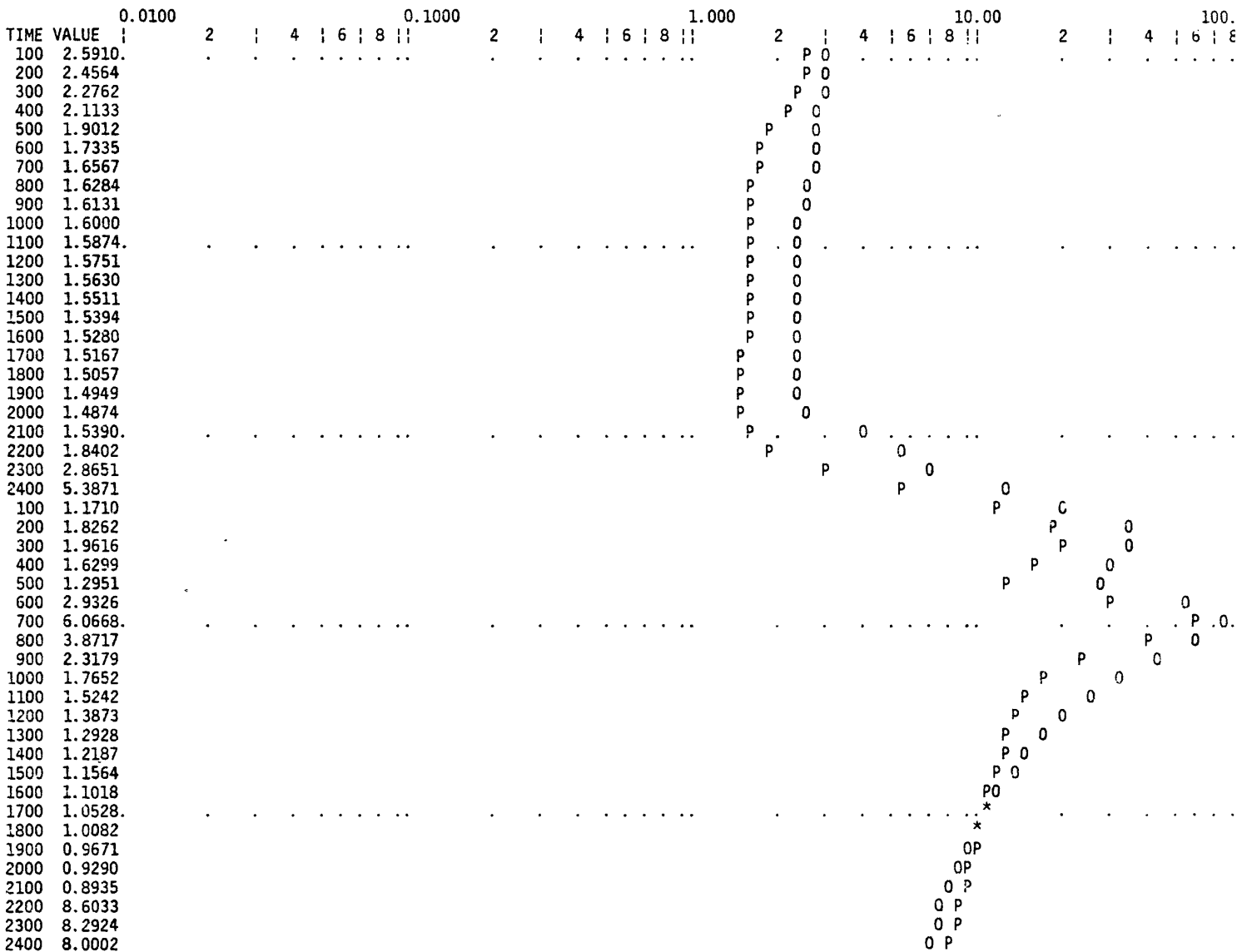
Figure II-8.--Line printer plot of simulated and observed discharge for storm 2 (March 13-14, 1956) on Cane Branch watershed.
