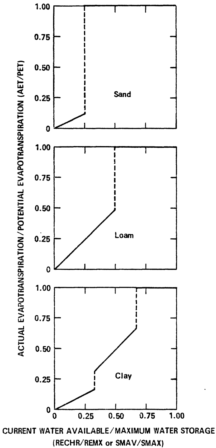
Figure 5.--Soil-water withdrawal functions for evapotranspiration (modified from Zahner, 1967).
