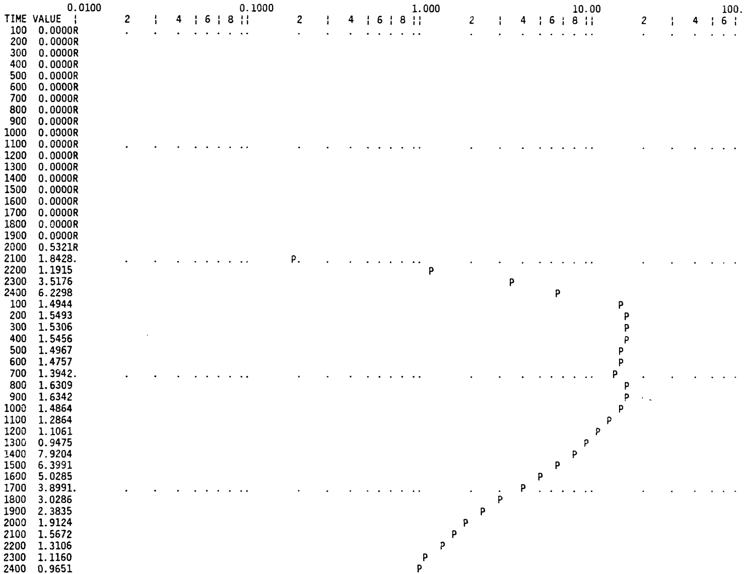
Figure 32.--Storm sediment-concentration plot.
