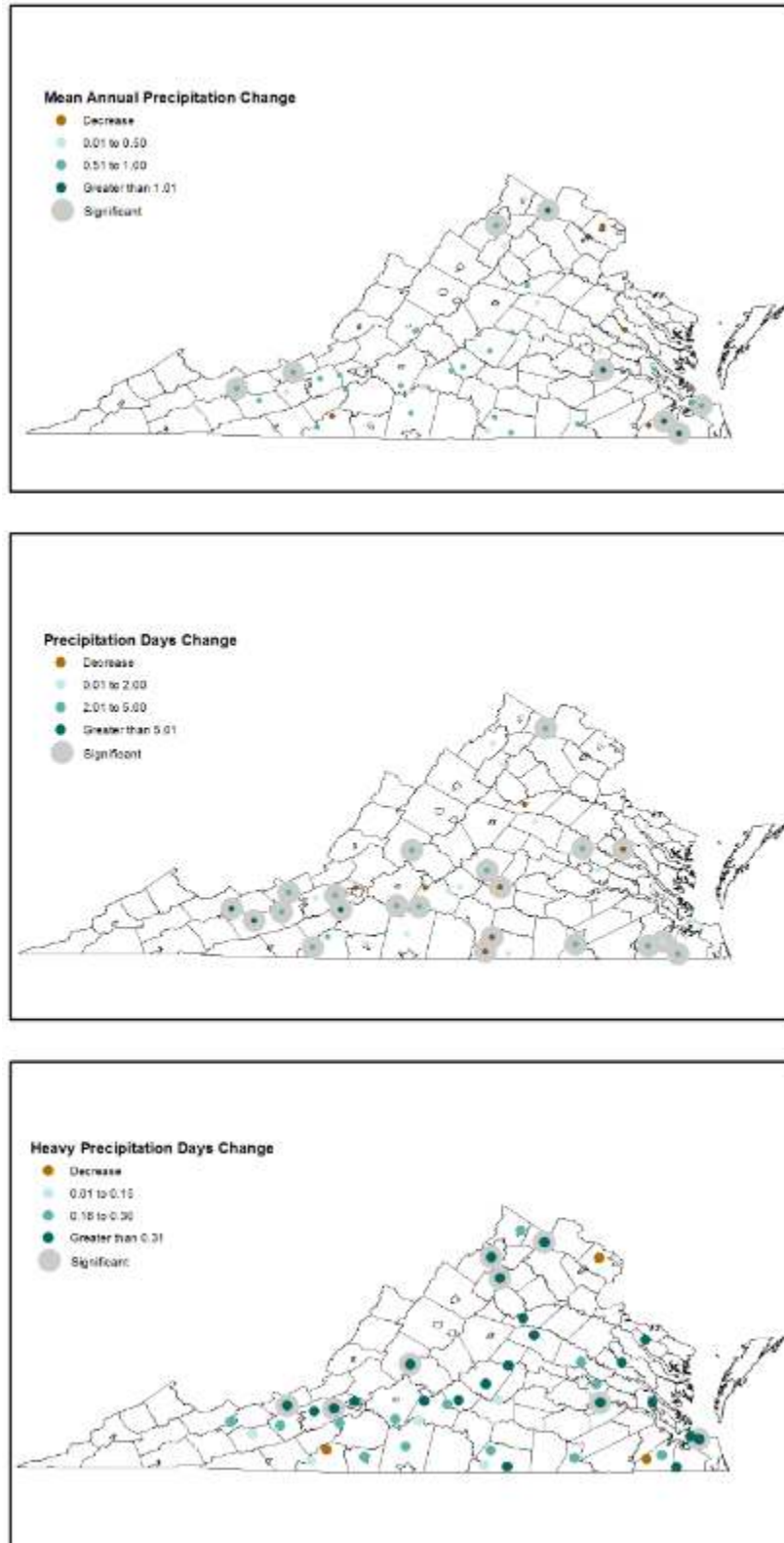
Figure 3. (top to bottom) Changes (decade -1 ) in total precipitation (inches), precipitation days, and heavy precipitation days (Appendix C).
