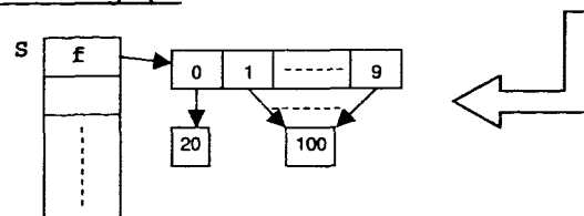
Figure 2. Combining numerical invariants and pointer analysis
