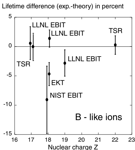
Fig. 3. Lifetime data for the 2s^2 2p^2 P_{3/2}^o level in the ground state of B-like ions from \text{Cl}^{12+} through \text{Ti}^{17+} . The data are normalized to the theoretical results given by Galavís et al. [89], which include a semi-empirical correction for experimental transition energies. A number of other theoretical results are within 0.6% of these values [71, 90–93]. The experimental data other than for Cl XIII [52] are from an electrostatic Kingdon trap (EKT) [22], from the NIST and LLNL electron-beam ion traps [73, 87, 88], and from the heavy-ion storage-ring TSR (74).
