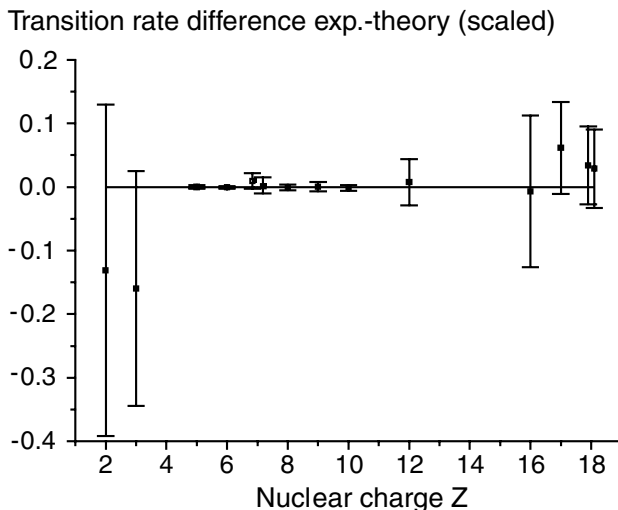
Fig. 2. Iso-electronic trend of the transition-rate data for the 1s^2\ ^1S_0-1s2s\ ^3S_1 magnetic dipole (M1) transition in He-like ions. Out of the full range of experimental data, Z = 2 to 54, only the low- Z range Z \leq 18 is shown. The particularly precise data for ions in the range 5 \leq Z \leq 10 underline the motivation for the present review: precise data are just so much more meaningful. Data for Z = 5 to 7 (leftmost entry) are from the heavy-ion storage ring TSR [38,39], exploiting dielectronic recombination processes for monitoring the excited level population. The other data for Z = 7 to 12 have been obtained by way of X-ray observations at the Livermore electron-beam ion trap EBIT-II [41–43]. All experimental data have been scaled by normalization to the results of the fully relativistic calculation by Johnson et al. [44], and only the deviations from this prediction are displayed. For a discussion of these particular measurements and for a comparison to other calculations, see ref. 43.
