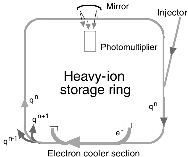
Fig. 1. Schematics of a heavy-ion storage ring with particle detection (bottom) and photon detection (top). To indicate the scale: the Heidelberg heavy-ion storage-ring circumference is 55 m, while the photomultiplier tube has a diameter of about 25 mm.
