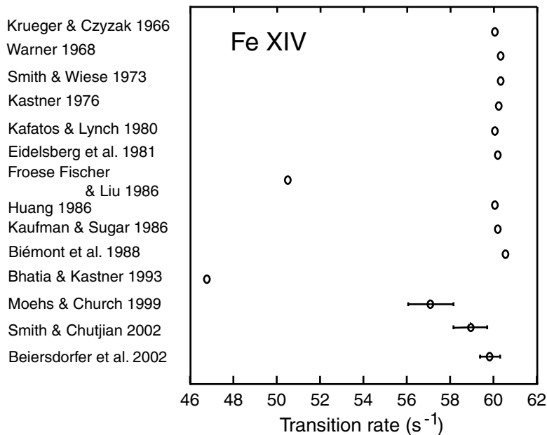
Fig. 4. Transition-rate data for the 3s^23p^2P_{3/2}^o level in the ground state of the Al-like ion Fe^{13+} . Note how most calculational results agree within a close interval with each other. The two deviating theoretical results apparently have not been adjusted for the experimental fine-structure intervals, clearly underlining the computational problems with that entity. The first (Texas A&M/Reno) electrostatic ion-trap measurement (by Moehs and Church) [24], however, did not resolve the evident discrepancy. The electron-beam ion-trap measurement at Livermore (by Träbert et al.) [77] clearly agrees with the (semi-empirically adjusted) majority of the predictions and settles the case, while the second (Caltech) electrostatic ion-trap measurement (by Smith and Chutjian) [95] has a result in between.
