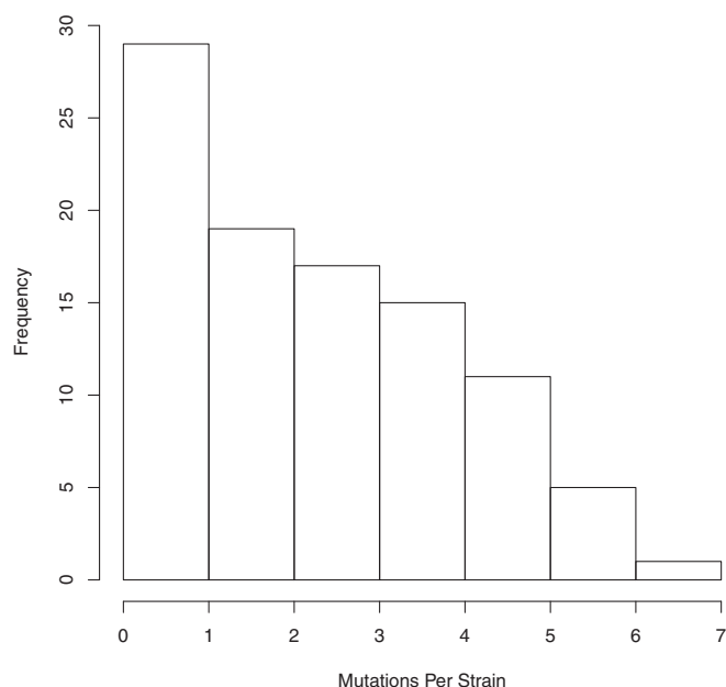
Fig. 1. Histogram of SNM counts per line in 97 MA lines with >60% of the genome covered to >8 \times read depth. Only positions sequenced to >8 \times read depth in all 97 lines were considered. A total of 256 SNMs were called in such regions in the 97 lines. Histogram shape may be Poisson ( P = 0.07 , G test) or negative binomial ( P = 0.1 , G test), but not binomial ( P < 0.001 , G test).
