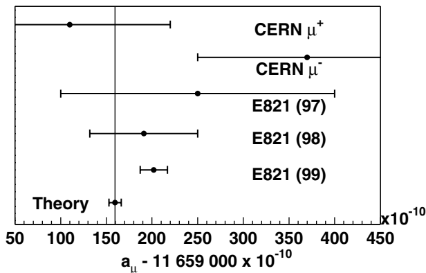
FIG. 5. Measurements of a_\mu and the standard model prediction with their total errors.
