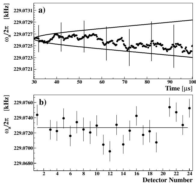
FIG. 4. (a) The fitted frequency \omega_a/2\pi vs start time of fit is shown together with representative error bars. The band indicates the size of expected statistical fluctuations. (b) Fits to the spectra from individual detectors. Detectors 2 and 20 were excluded from the \omega_a analyses because of a readout problem and a miscalibration, respectively.
