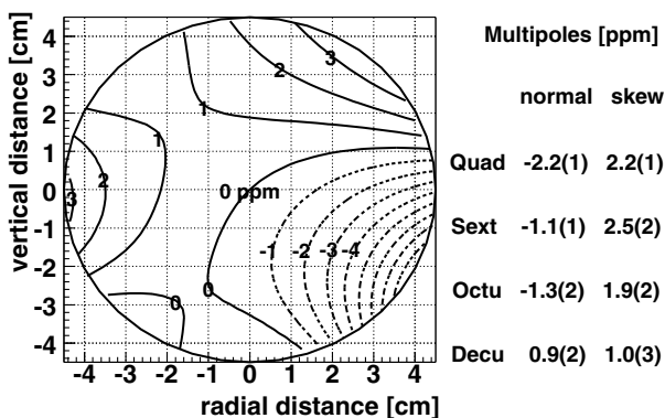
FIG. 1. A two-dimensional multipole expansion of the field averaged over azimuth from one out of seventeen trolley measurements. One ppm contours are shown with respect to a central azimuthal average field B_0 = 1.451266 T. The circle indicates the muon beam storage region. The multipole amplitudes at the beam aperture radius of 4.5 cm are given.
