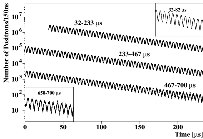
FIG. 3. Positron time spectrum overlaid with the fitted 10-parameter function ( \chi^2/\text{d.o.f.} = 3818/3799 ). The total event sample of 0.95 \times 10^9 e^+ with E \geq 2.0 GeV is shown.
