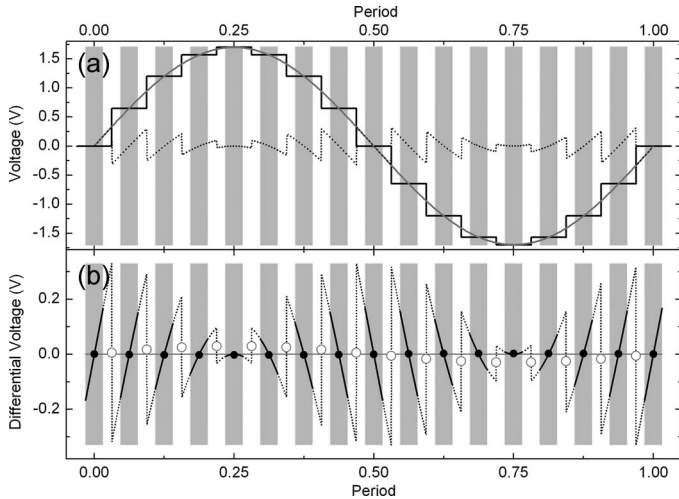
Fig. 2. (a) Ideal simulated ACPJVS staircase-approximated sine wave with 16 samples and ac source sine wave (both with 1.2 V rms amplitude and zero relative phase). The resulting differential waveform is represented by the dotted line. The gray and white stripes correspond to the different integration windows of the sampling voltmeter. (b) Zoom of the differential waveform. The circles show the magnitude of the integrated voltage for each sampling window. Free of transients, the solid circle samples are used for waveform amplitude reconstruction. The open circle samples that contain the transients are discarded.
