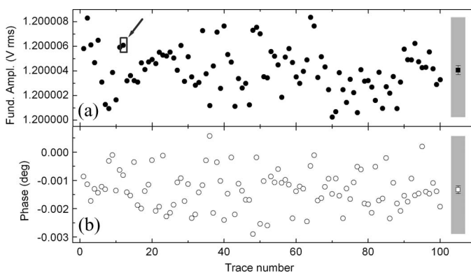
Fig. 4. Calculated values of the Fluke 5720A rms amplitude and phase (nominally 1.2 V and 0^\circ ) at 50 Hz inferred from the measured differential signal by use of an 80-step ACPJVS reference waveform. (a) Mean amplitude of the fundamental for each of the 100 traces. (b) Mean phase relative to the sampling window for the same sampled data. In each gray rectangle, we graphically report the resulting average value calculated over the 100 traces. The error bar represents the standard deviation of the mean ( k = 2 ). The arrow indicates the mean value of trace #12, whose detailed measurements are shown in Fig. 3.
