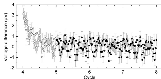
Fig. 8. Difference between the expected Josephson rms voltage (10 mV) and the amplitude measured with the sampling voltmeter as a function of time (50 Hz cycle). During cycles 1 through 4, the 100 mV range of the sampling voltmeter is overloaded with the 1.2 V juxtaposed waveform. After a complete cycle (open circles), the sampler fully recovers from the overloaded state (solid circles).
