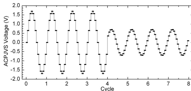
Fig. 7. Example of a dual juxtaposed ACPJVS waveform with n = 4 cycles of a 1.2 V rms and m = 4 cycles of 0.5-V rms sine waves, with a relative phase of 30^\circ . For clarity, we show a waveform with only 16 samples per cycle.
