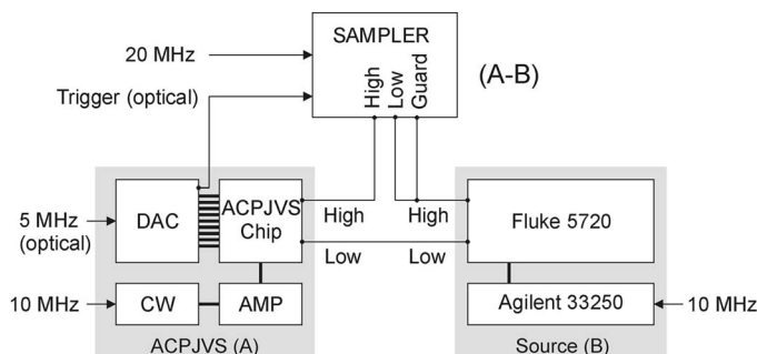
Fig. 1. Diagram showing the differential (A–B) measurement setup. The reference signal (a square wave at the same frequency of the ACPJVS waveform) for the phase and frequency locking of the Fluke 5720A is provided by an Agilent 33250 arbitrary waveform generator. All clock signals are locked to the same reference. The guard of the sampling voltmeter is driven by the same signal (B) as the low input of the sampler. Glossary for the ACPJVS system: DAC = Current bias electronics, AMP = microwave amplifier, and CW = 18.3 GHz microwave generator.
