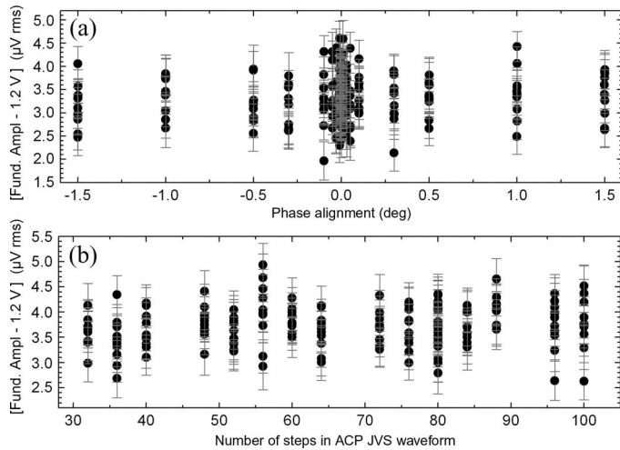
Fig. 5. Demonstration that the differential sampling method produces consistent results with regard to (a) phase misalignment and (b) number of steps in the ACPJVS waveform.
