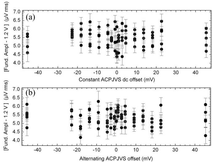
Fig. 6. Demonstration that the differential sampling method produces consistent results with regard to (a) ACPJVS dc offsets and (b) ACPJVS interleaved offsets.
