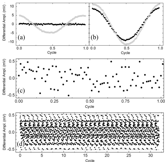
Fig. 3. Differential amplitudes measured by the sampling voltmeter using an ACPJVS stepwise-approximated 50 Hz 1.2 V rms sine wave with 80 steps per period, (a) with zero relative phase and (b) with 0.3^\circ relative phase for “on-step” (solid circles) and transient (open circles) samples. The measured amplitudes of only the “on-step” samples for (c) the first cycle and (d) all 32 cycles of the zero relative phase trace. The two horizontal lines in (d) indicate the maximum amplitudes measured and emphasize a small amplitude modulation.
